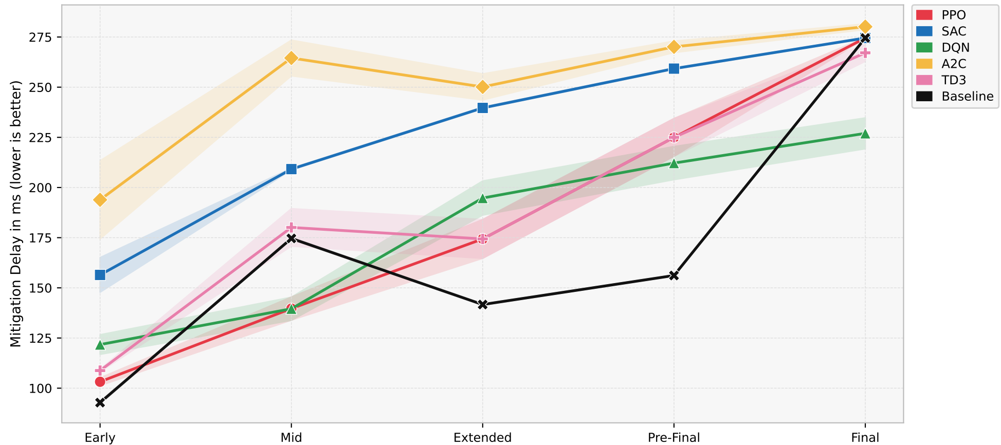
Mitigation Delay Across Attack Phases (mean \pm 95% CI, 3 seeds)
