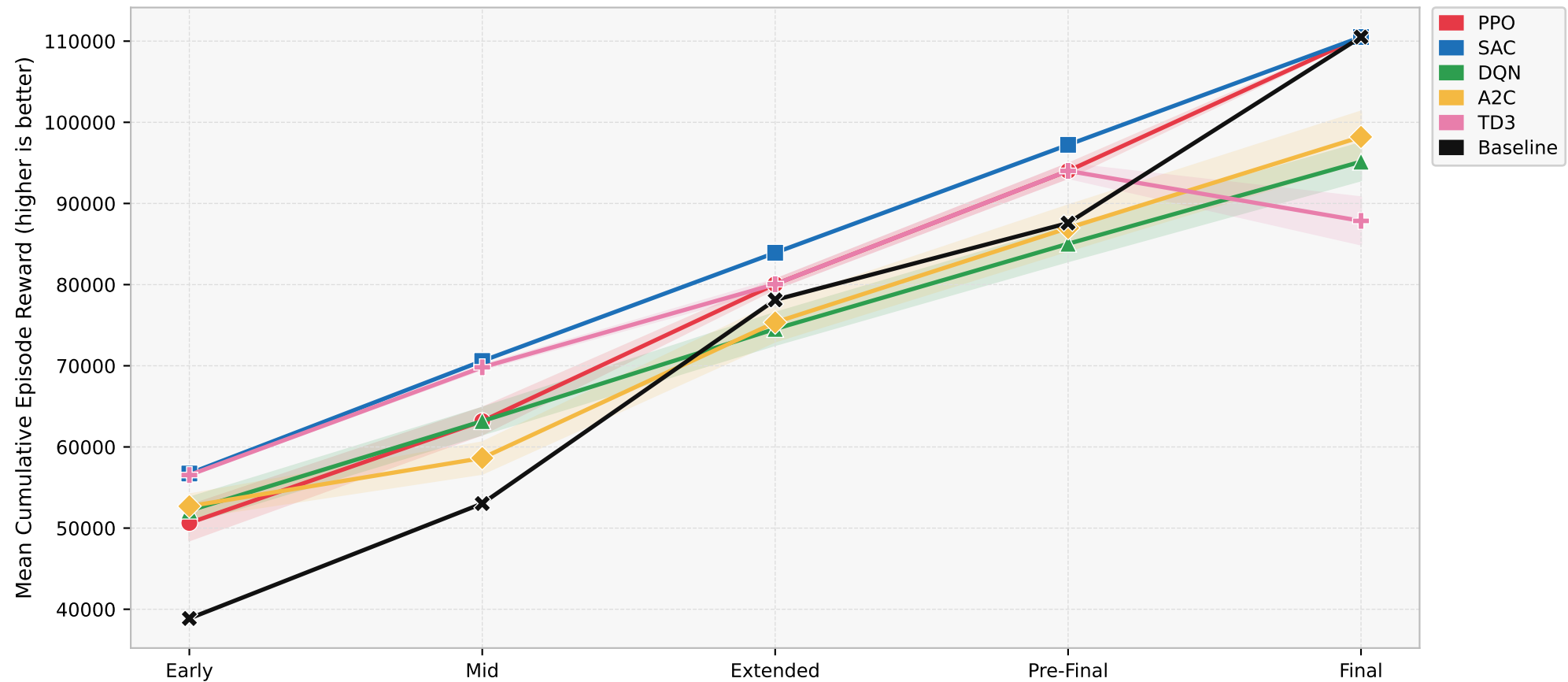
Mean Episode Reward Across Attack Phases (mean \pm 95% CI, 3 seeds)
