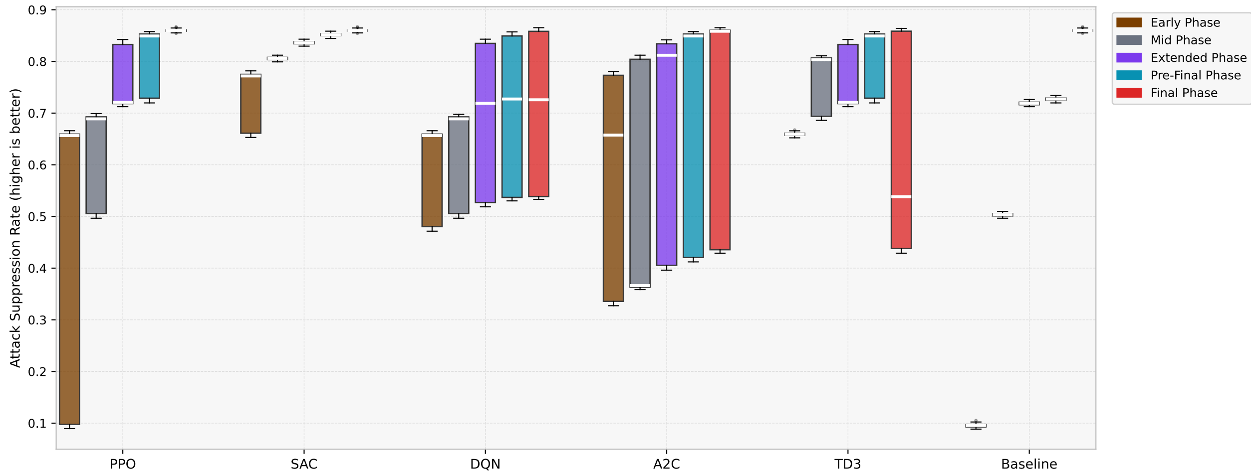
Cross-Seed Variance in Attack Suppression Rate (3 seeds x evaluation episodes)
