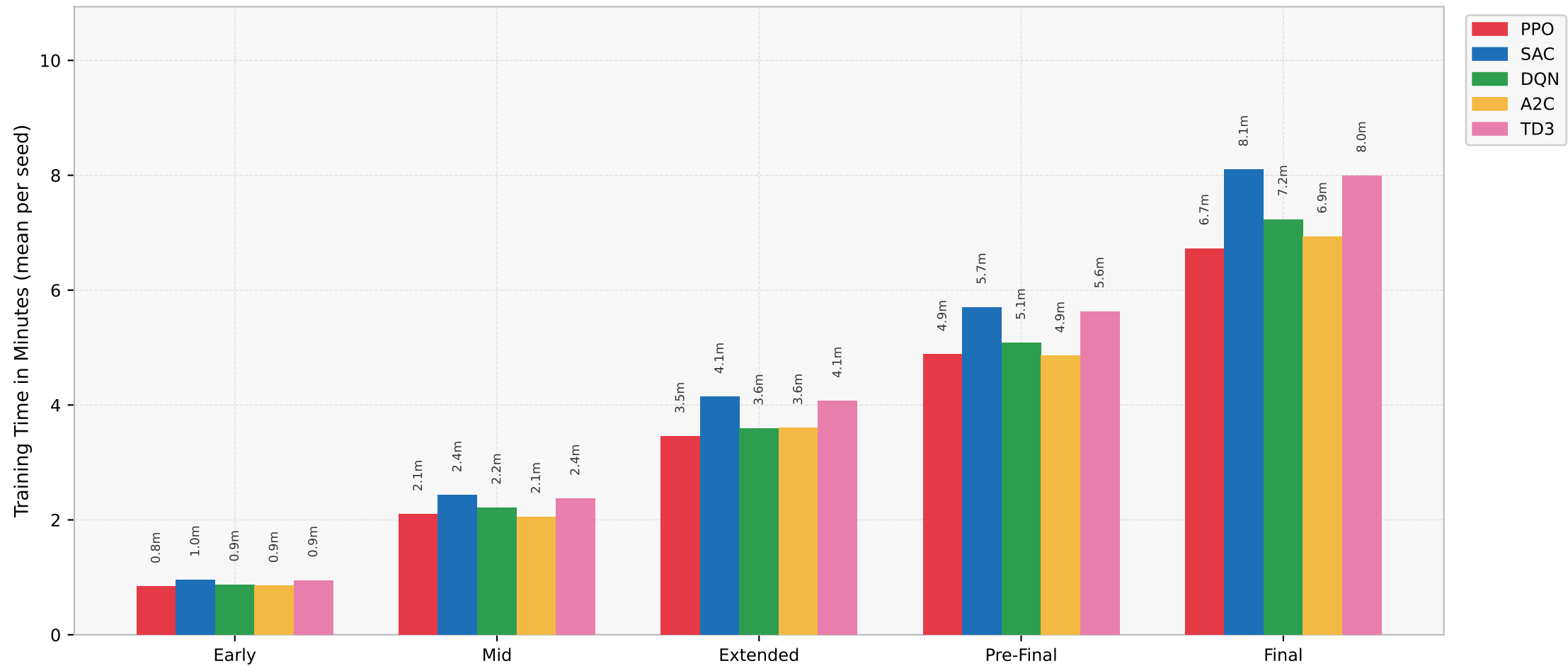
Algorithm Training Time per Phase (Baseline excluded - no learning)
