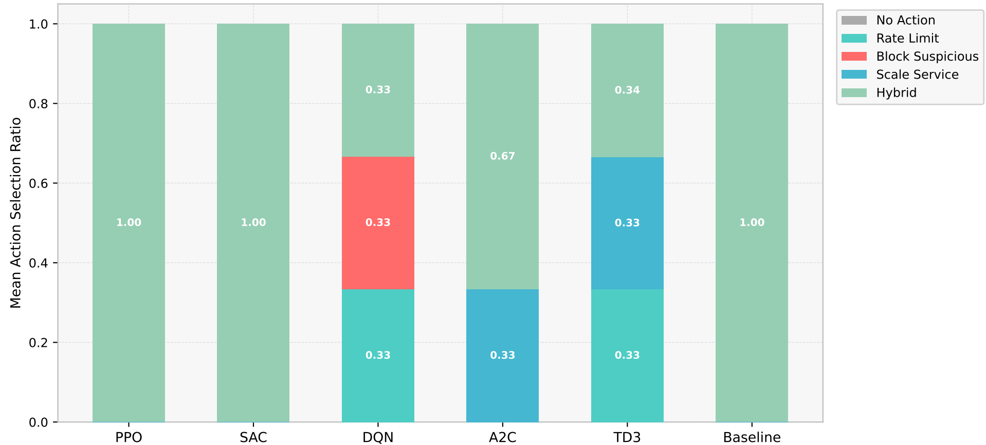
Mitigation Action Distribution - Final Phase (attack rate 0.88)
