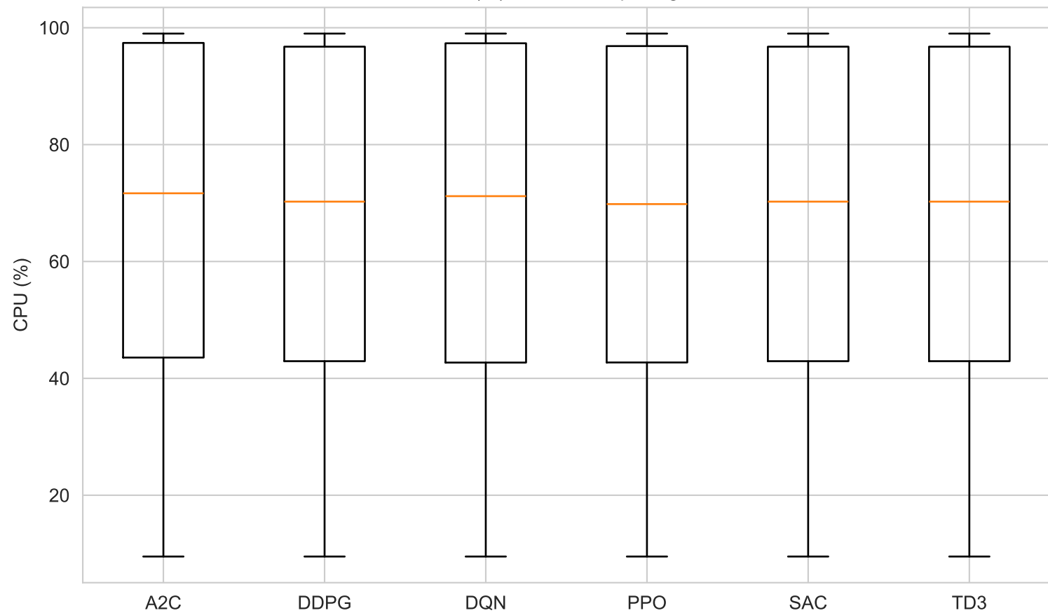
CPU (%) Distribution per Agent
