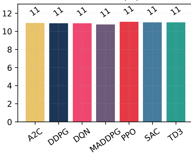
Efficiency (Thr/CPU)
