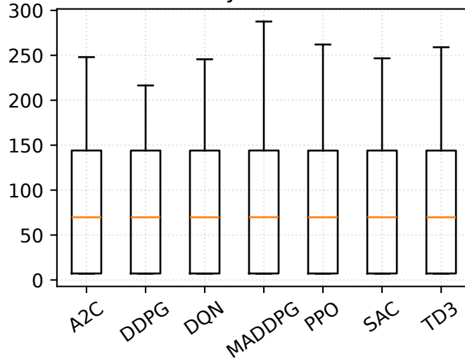
Latency Distribution
