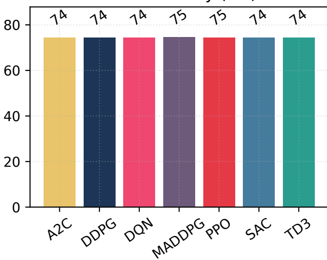
Mean Memory (%)
