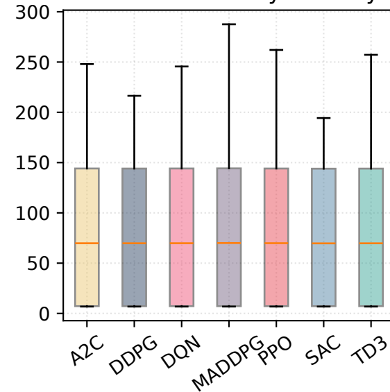
Fault Occurrence Distribution
