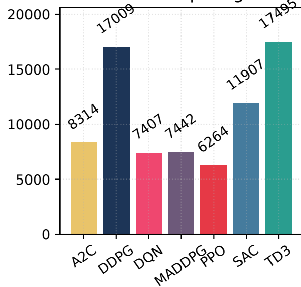
Latency During Faults
