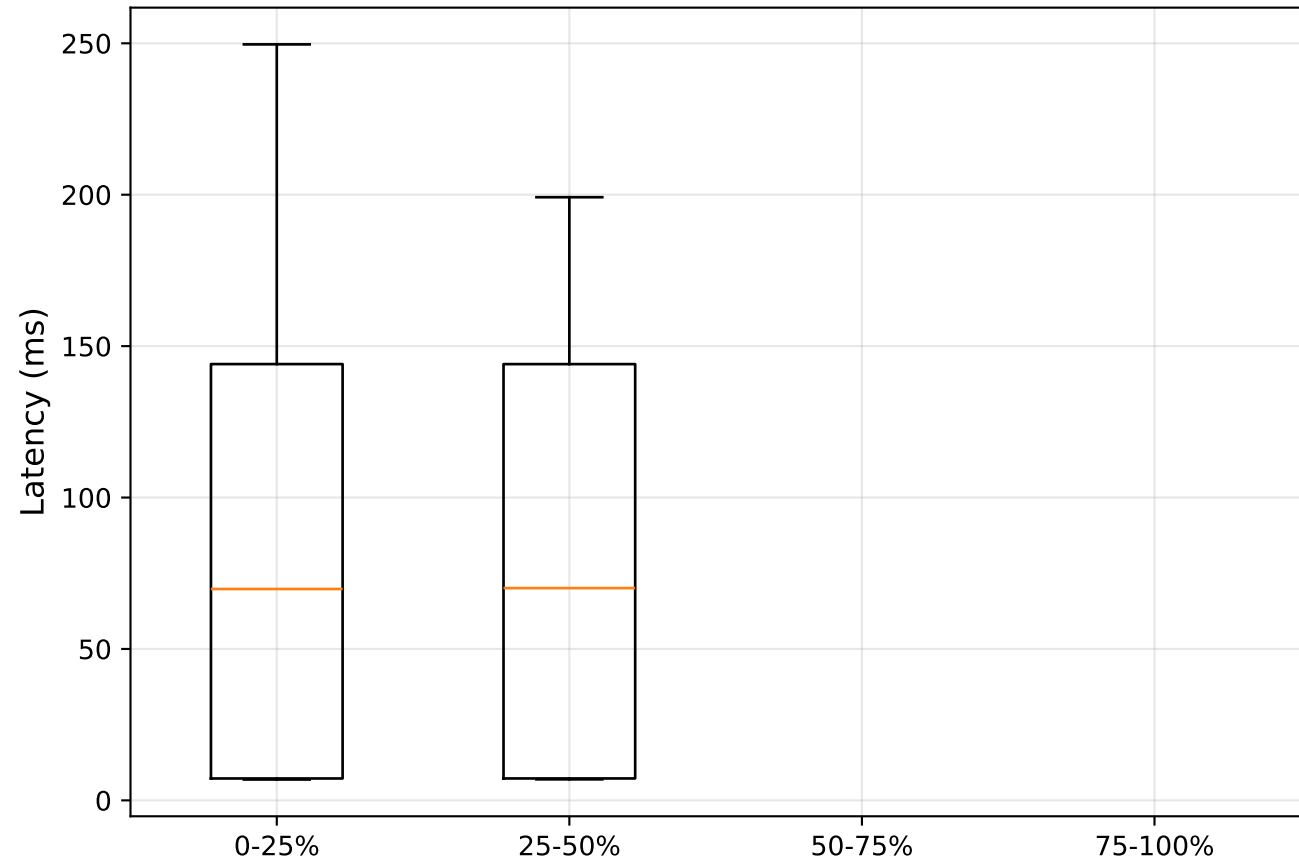
Latency by CPU Load (early)
