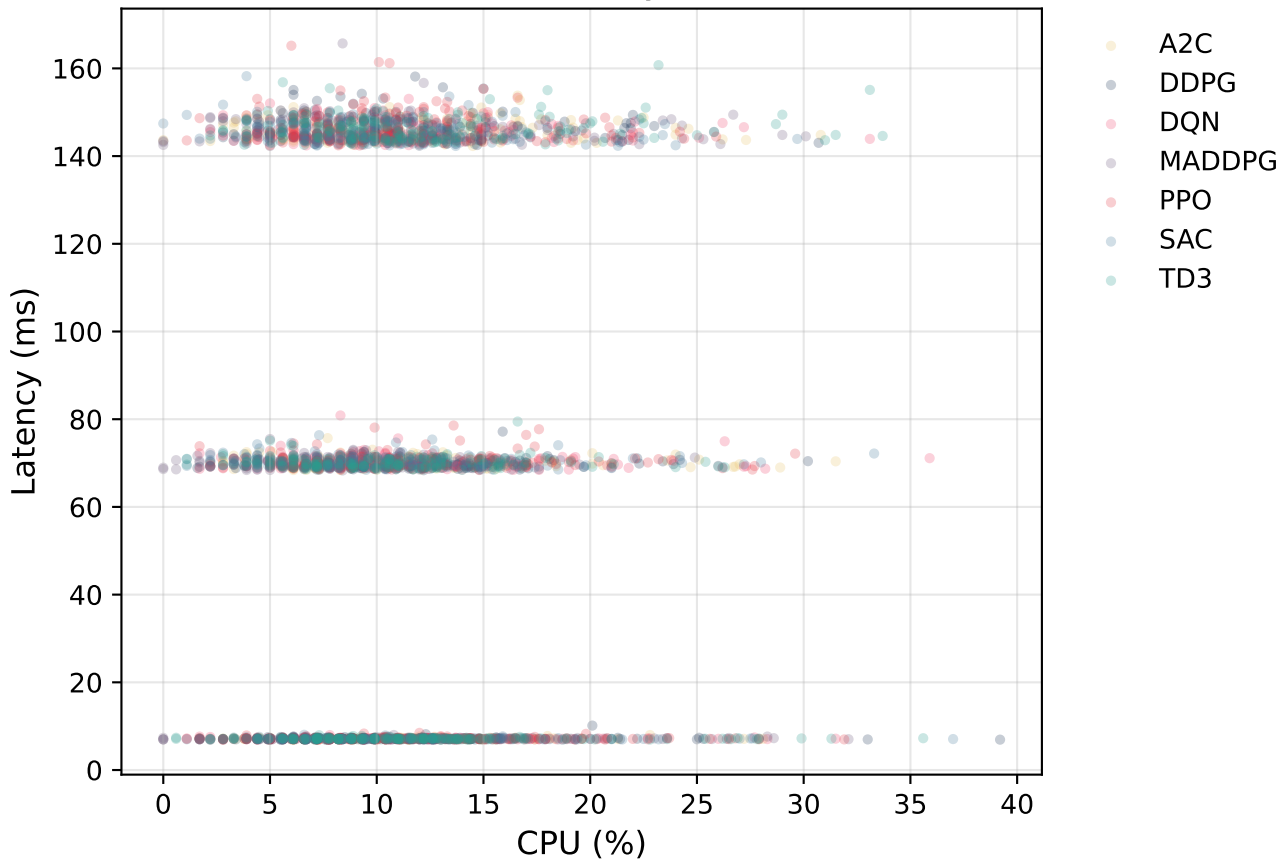
CPU vs Latency (final)
