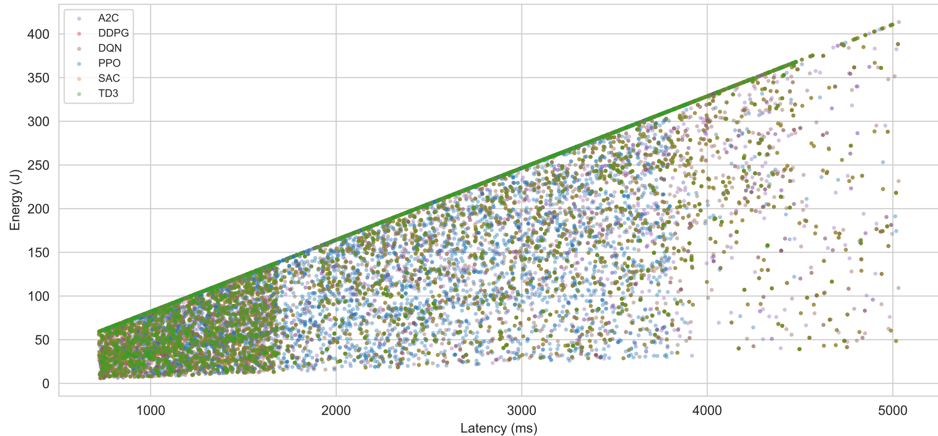
Energy–Latency Pareto (Downsampled)
