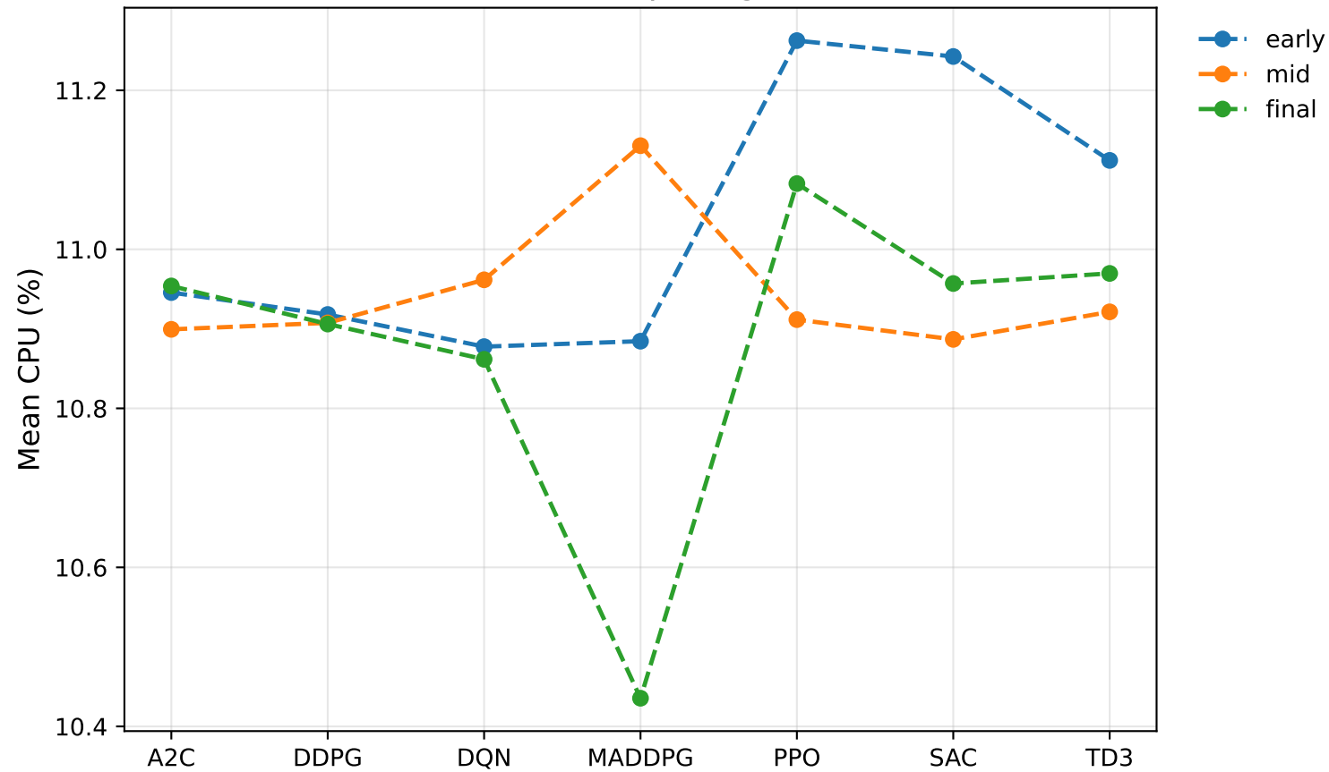
Mean CPU per Agent
