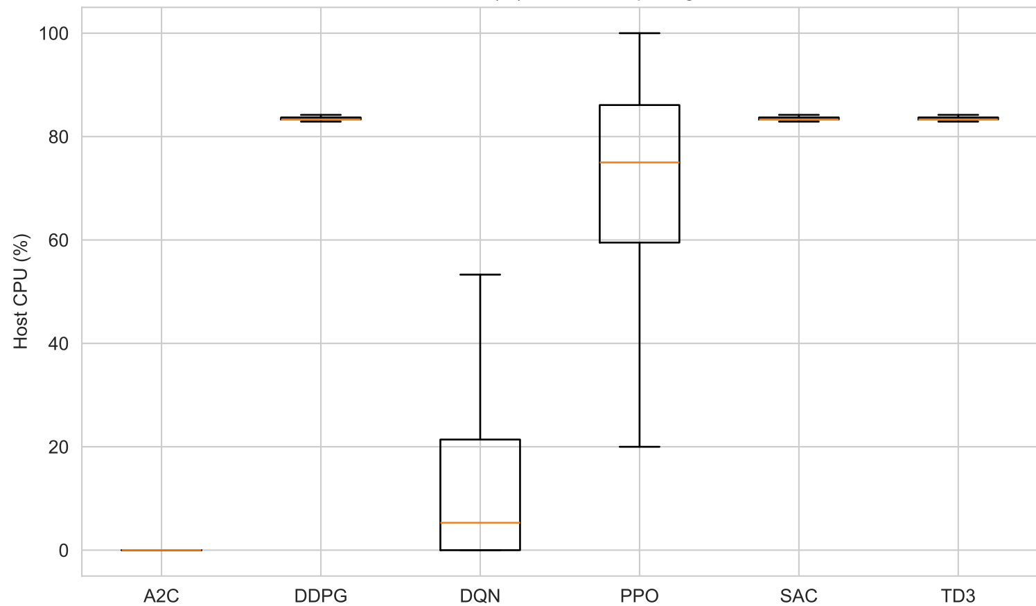
Host CPU (%) Distribution per Agent
