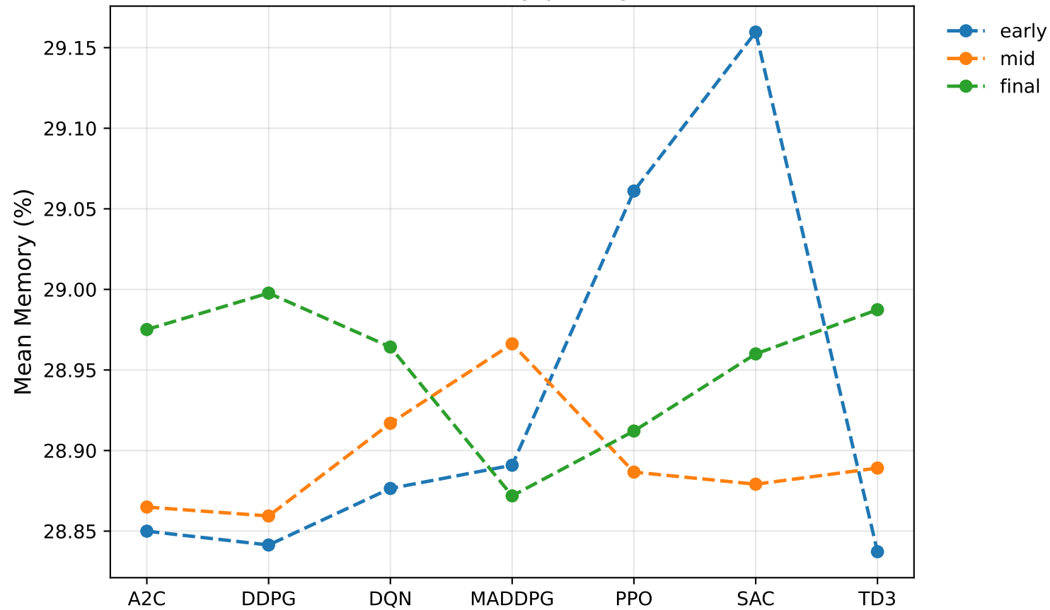
Mean Memory per Agent
