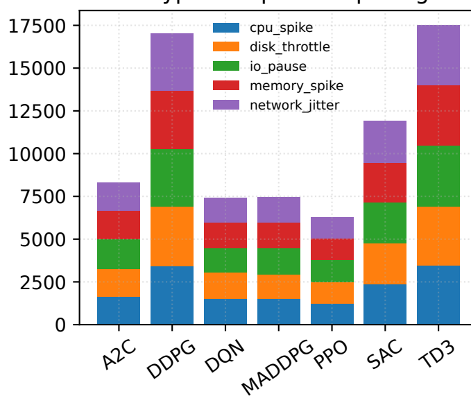
Faults per 1000 Episodes
