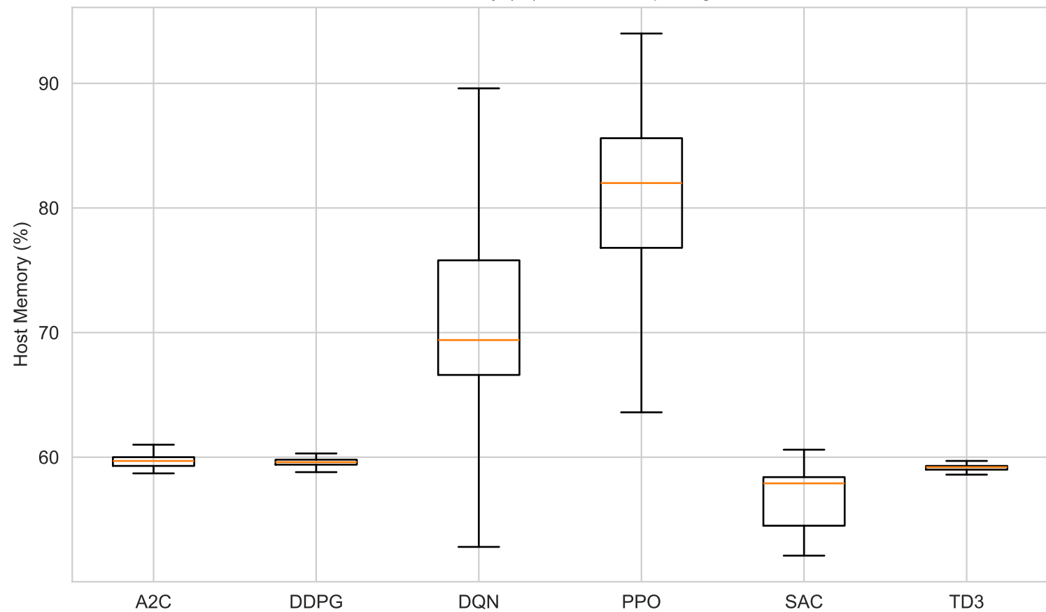
Host Memory (%) Distribution per Agent
