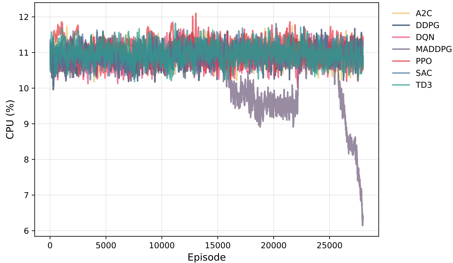
CPU (%) Trend (final)
