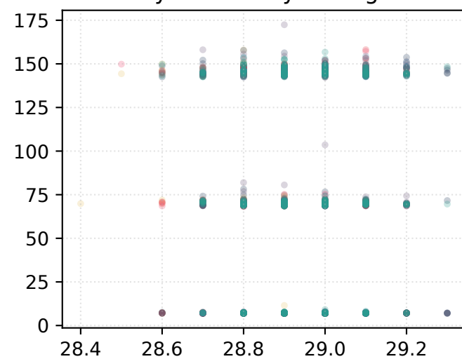
Memory vs Latency During Faults
