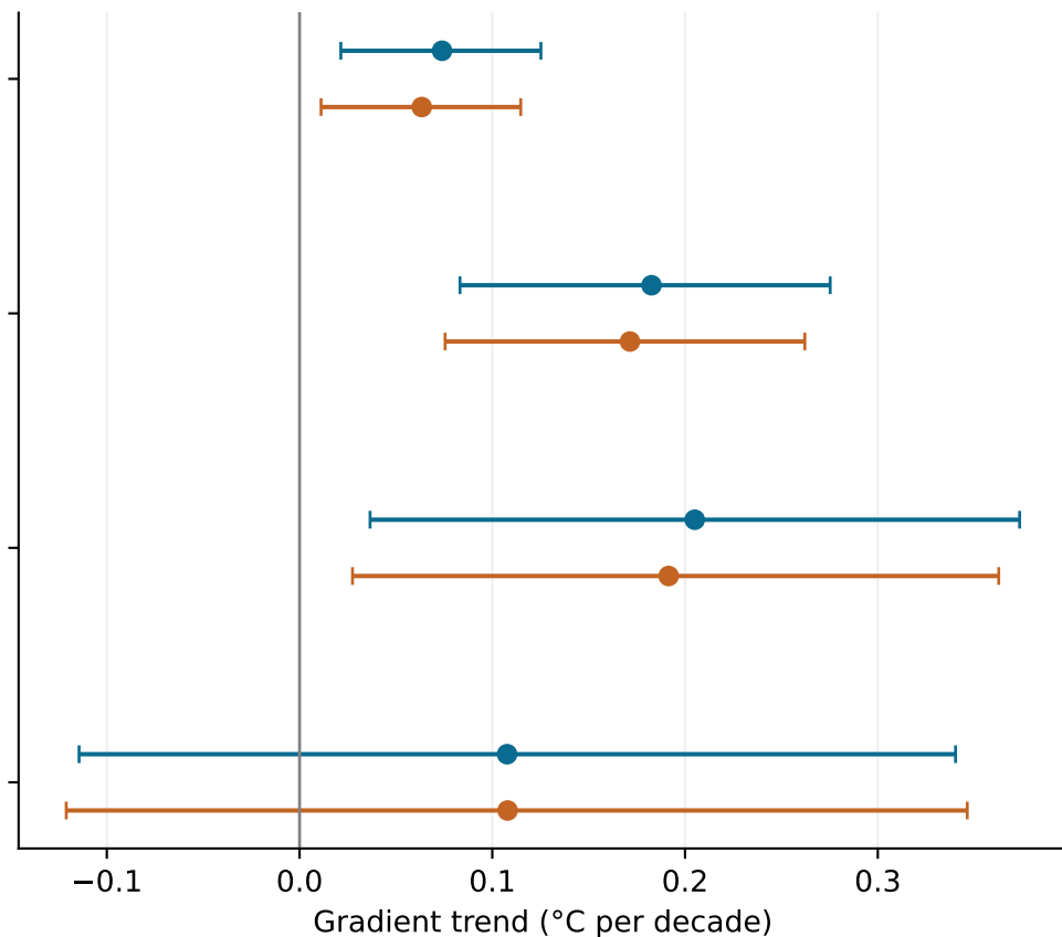
Latitude: 5°S-5°N
