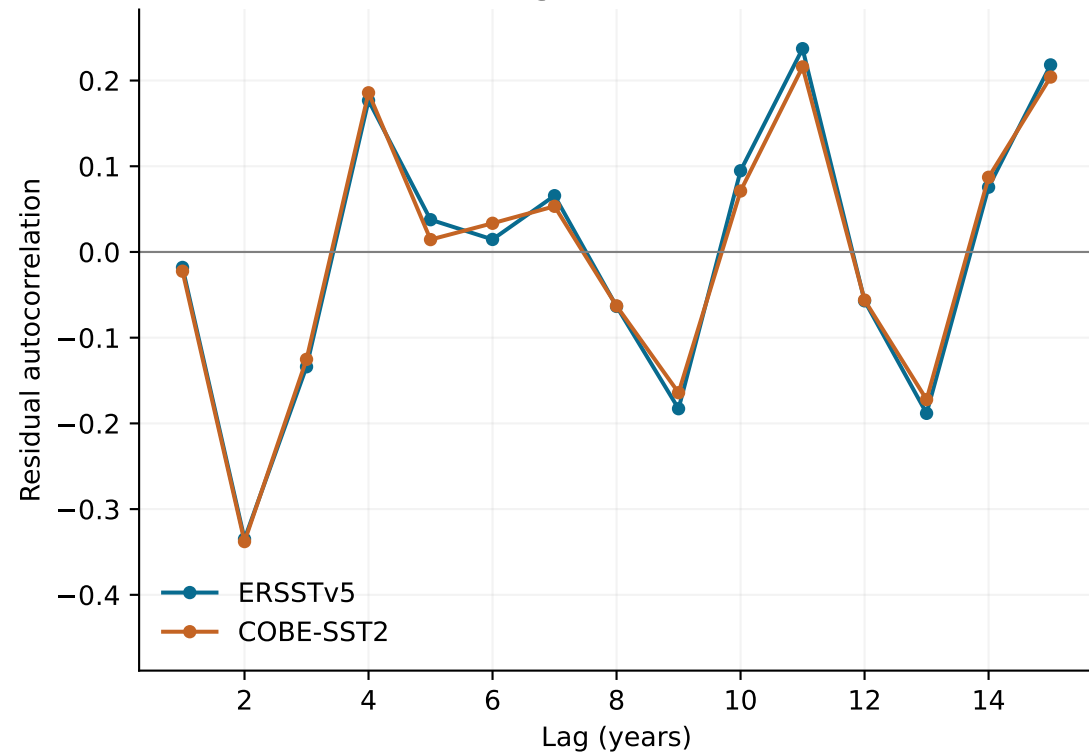
Detrended gradient, 1950-2025
