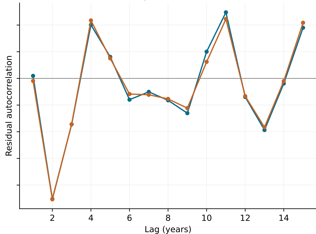
Detrended gradient, 1979-2025
