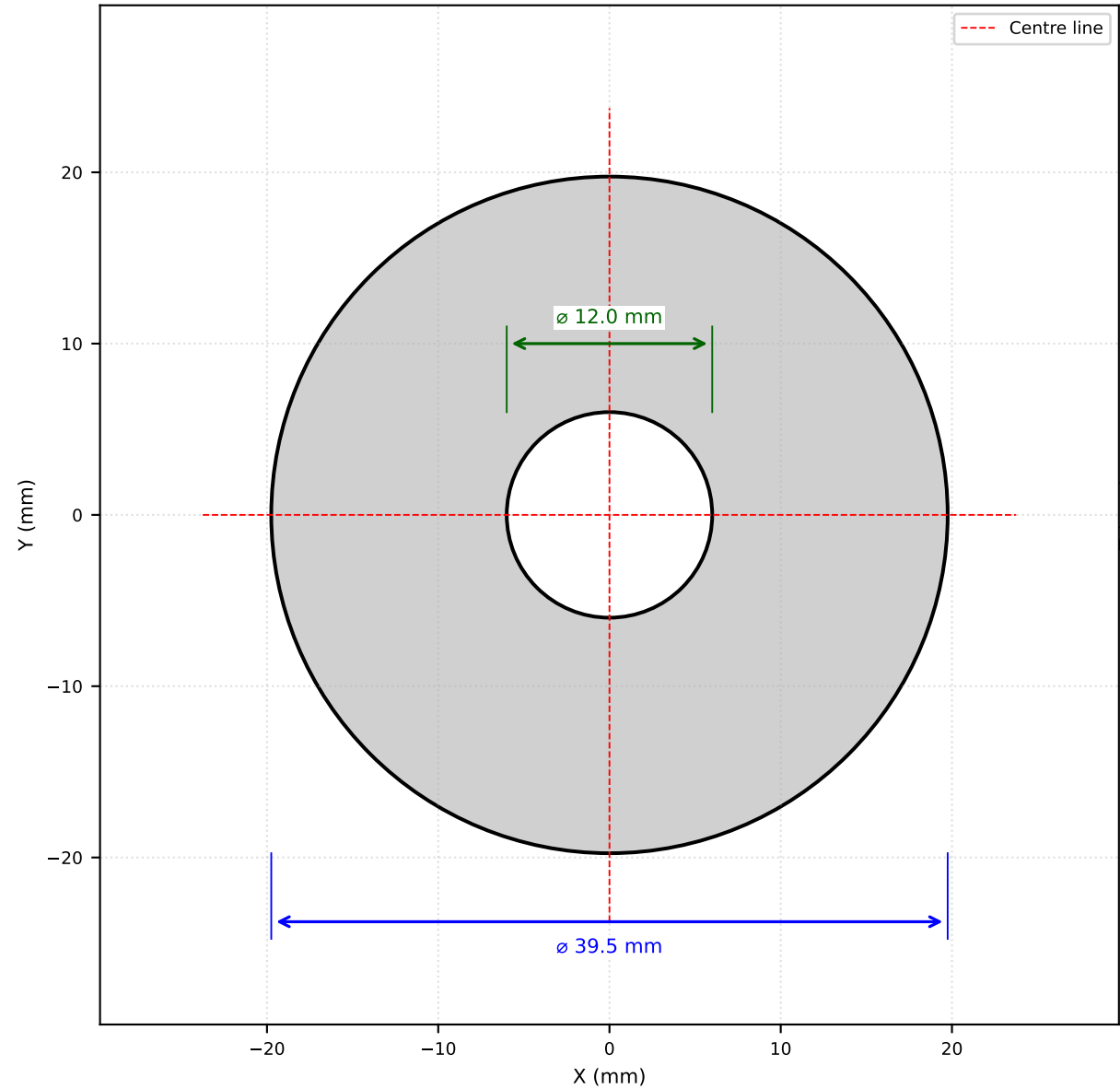
TOP VIEW (Plan)
