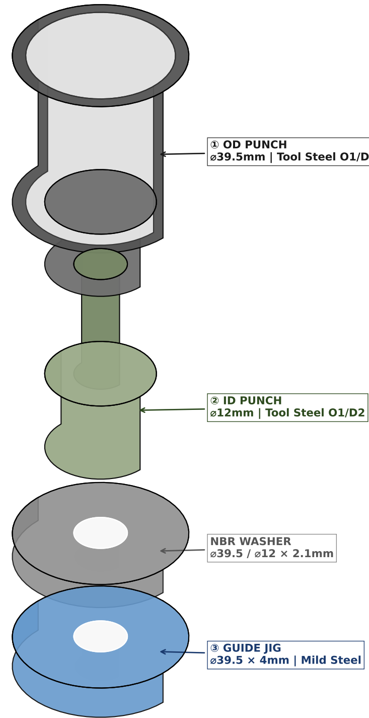
ISOMETRIC VIEW — Assembly (Exploded)
