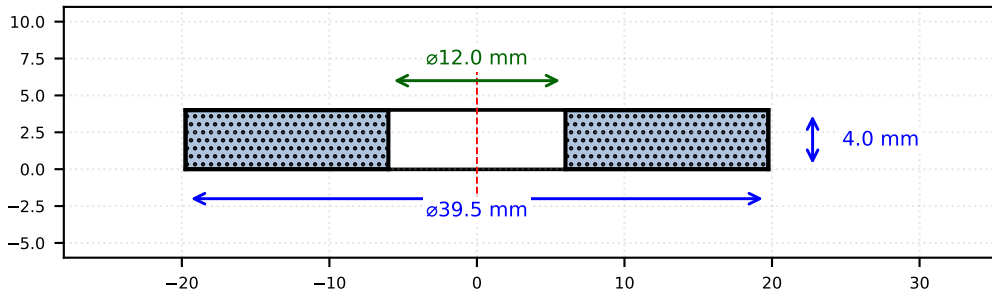
ITEM 3 — GUIDE JIG (Cross-section) Mat: Mild Steel / Aluminium
