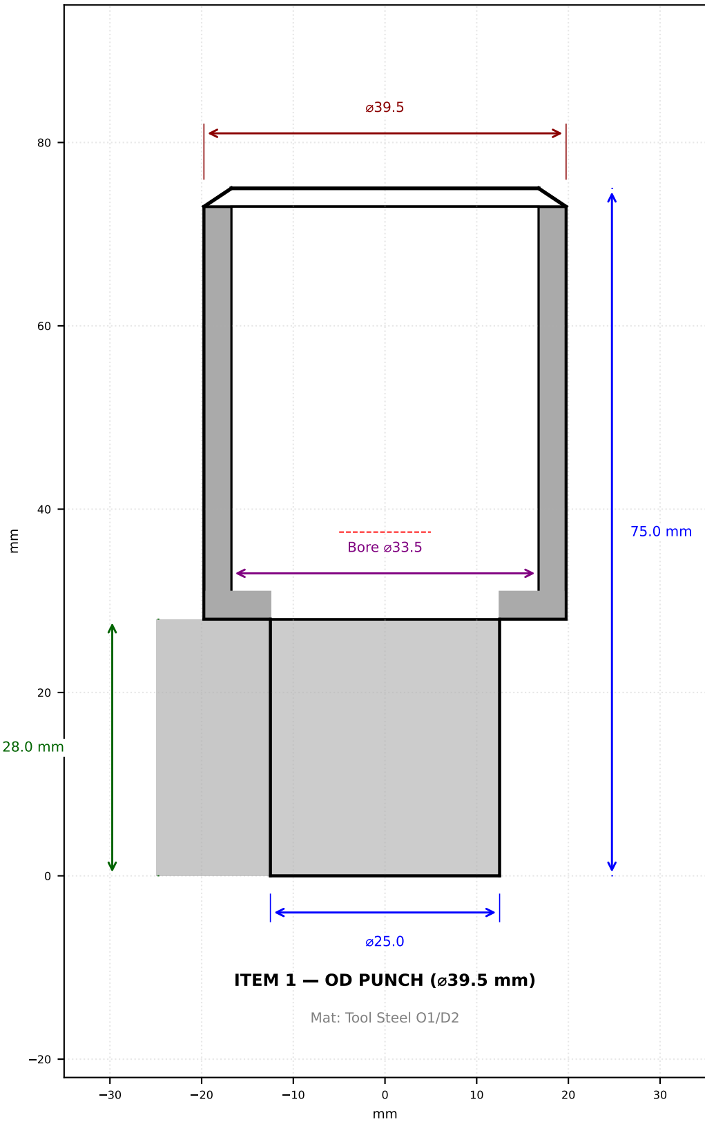
FRONT VIEW — OD Punch
