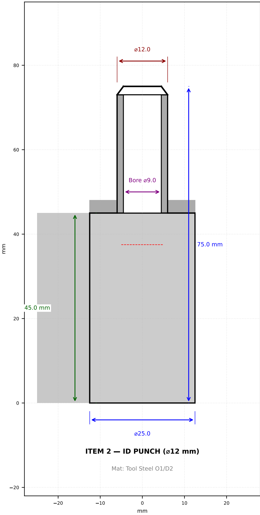
FRONT VIEW — ID Punch
