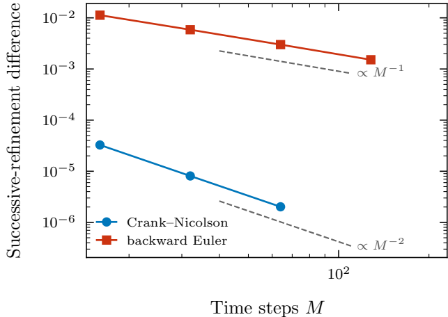
(b) Temporal convergence (MMS)
