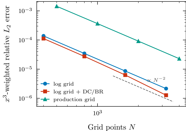
(a) Spatial convergence (MMS)
