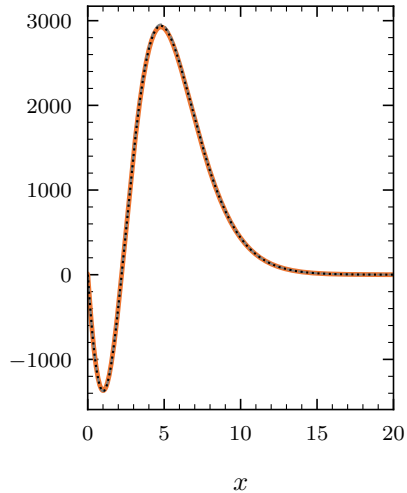
Peaked power-law
