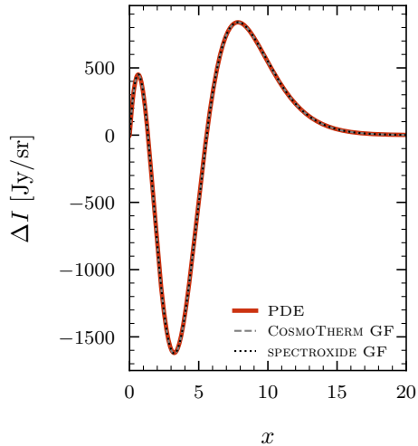
Sinusoidal heating/cooling
