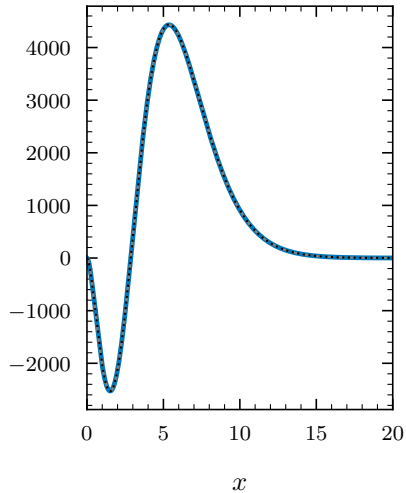
Wide Gaussian
