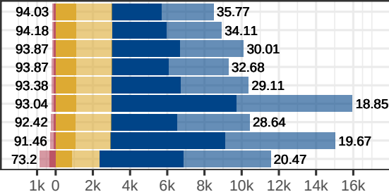
HCC1937
