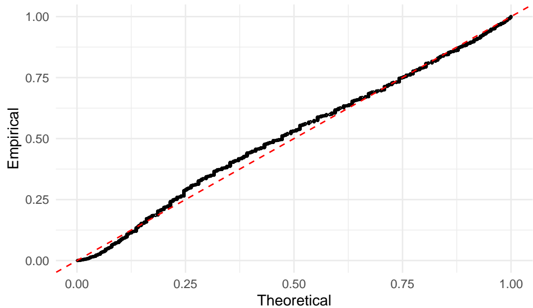
P-P Plot of VC9
