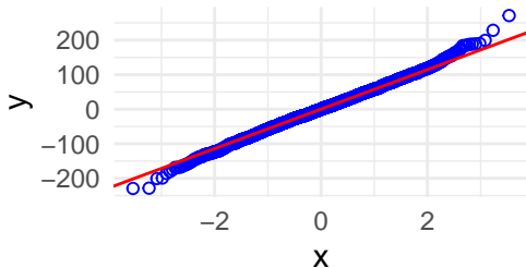
Q-Q Plot of Residuals
