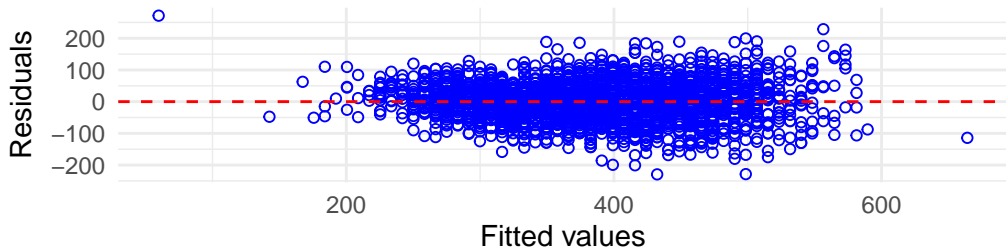
Residuals vs Fitted
