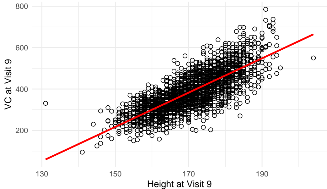
VC9 vs Height9 ( R^2 = 61.98\% )
