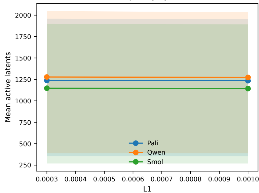
E. Sparsity by L1
