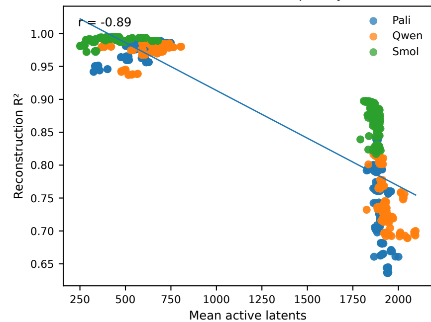
C. Reconstruction vs sparsity
