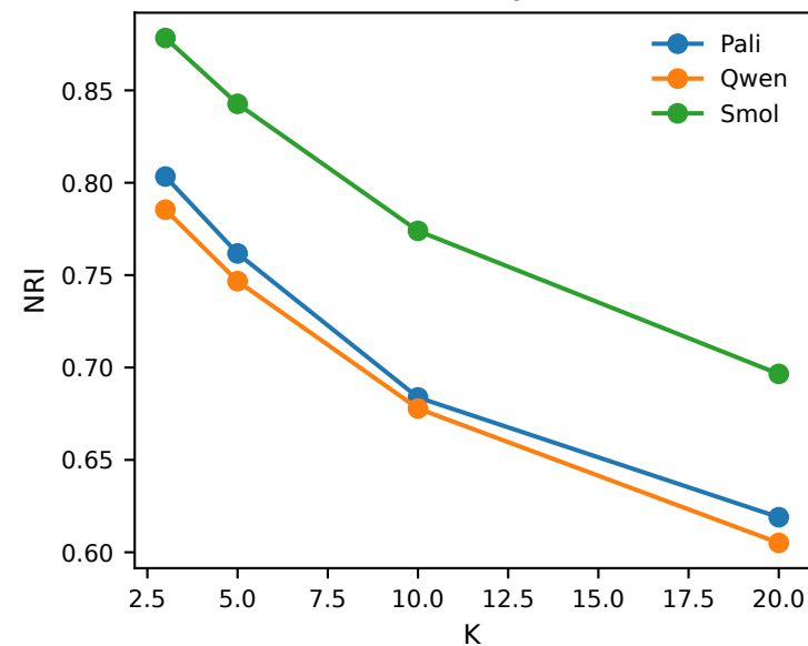
E. K-sensitivity of NRI
