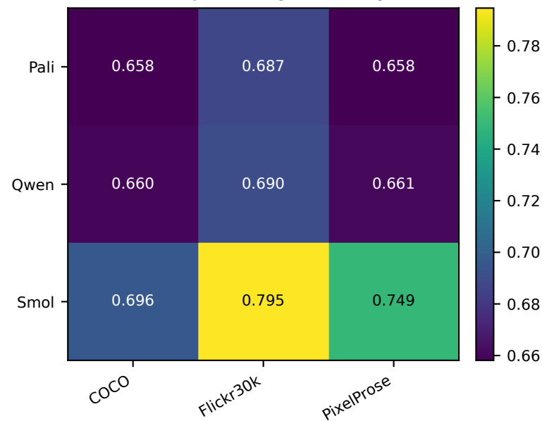
E. K-sensitivity of NRI
