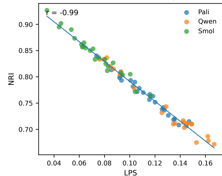
C. LPS-NRI consistency
