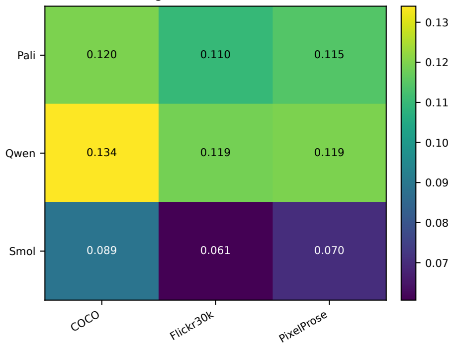
D. Shared-neighbor ratio
