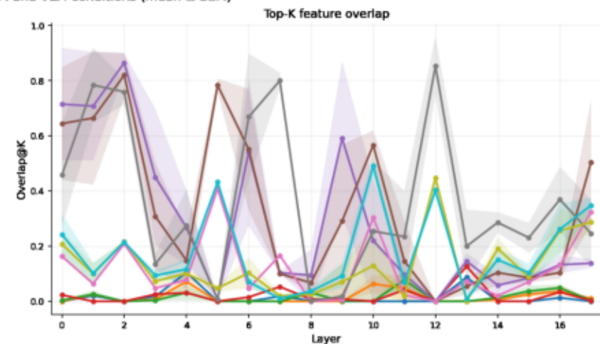
Layerwise superposition across LLM and VLM conditions (mean \pm SEM)
