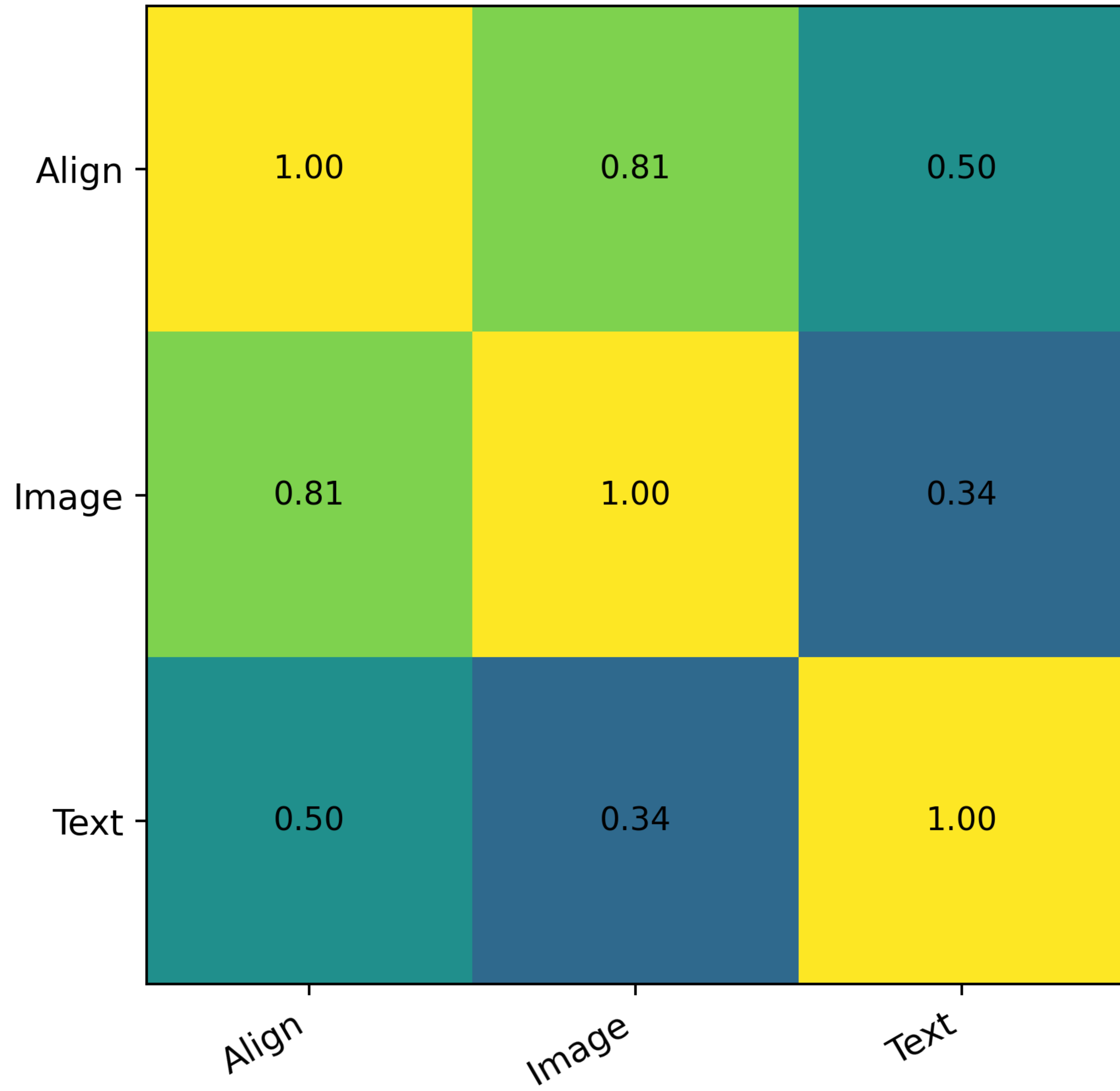
qwen2_vl pixelprose, layer 21
