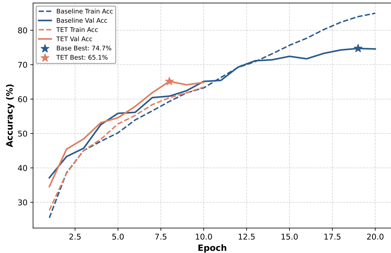
Training & Validation Accuracy (Generalization Gap)
