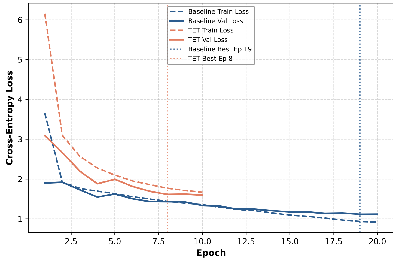
Training & Validation Loss (Overfitting Diagnostic)
