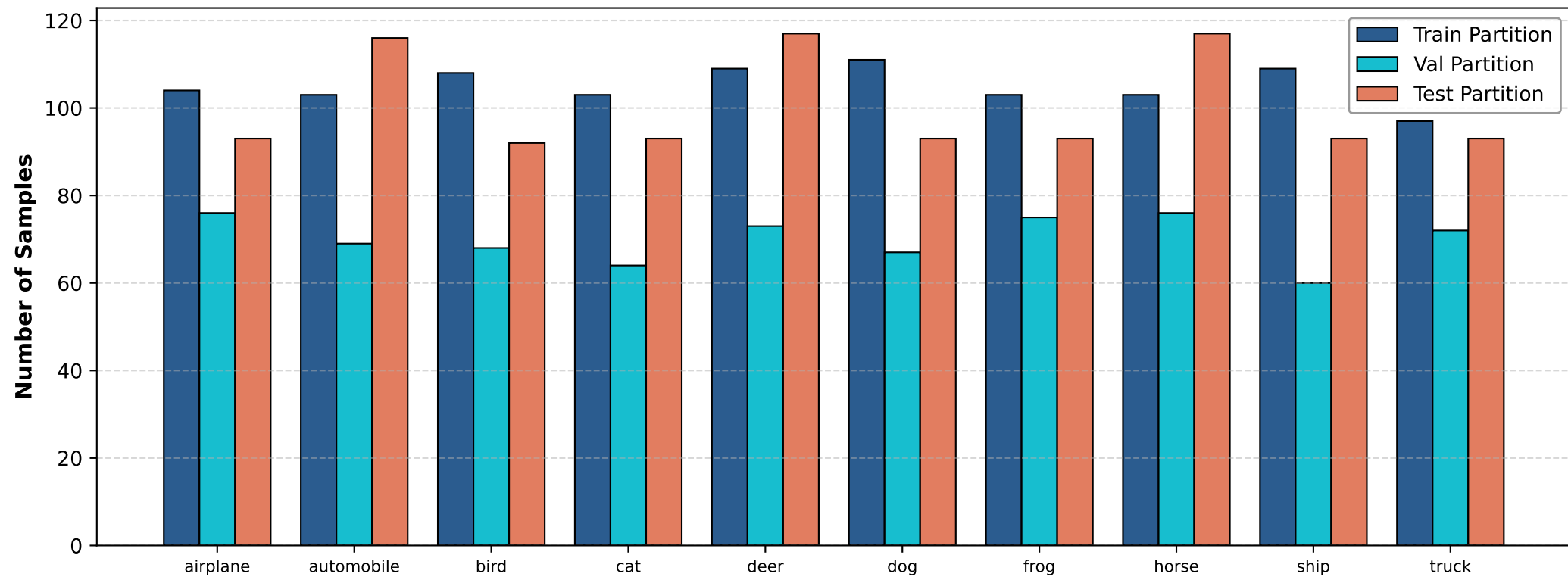
CIFAR10-DVS - Partitioned Class Distribution (Zero Leakage)
