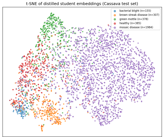
Fig. 2. t-SNE projection of the distilled student’s 1024-dimensional penultimate embeddings on the Cassava single-split test set. The majority mosaic disease class separates cleanly, while the minority classes overlap, mirroring the per-class scores (Table IX) and the confusion matrix (Figure 1).
