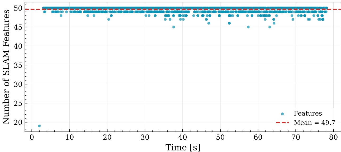
SLAM Feature Count Over Time
