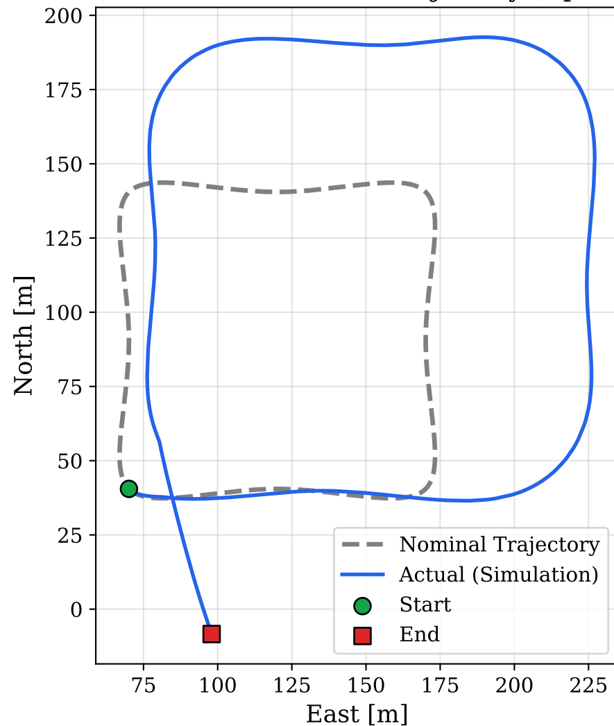
Nominal vs. Simulation Trajectory (square)
