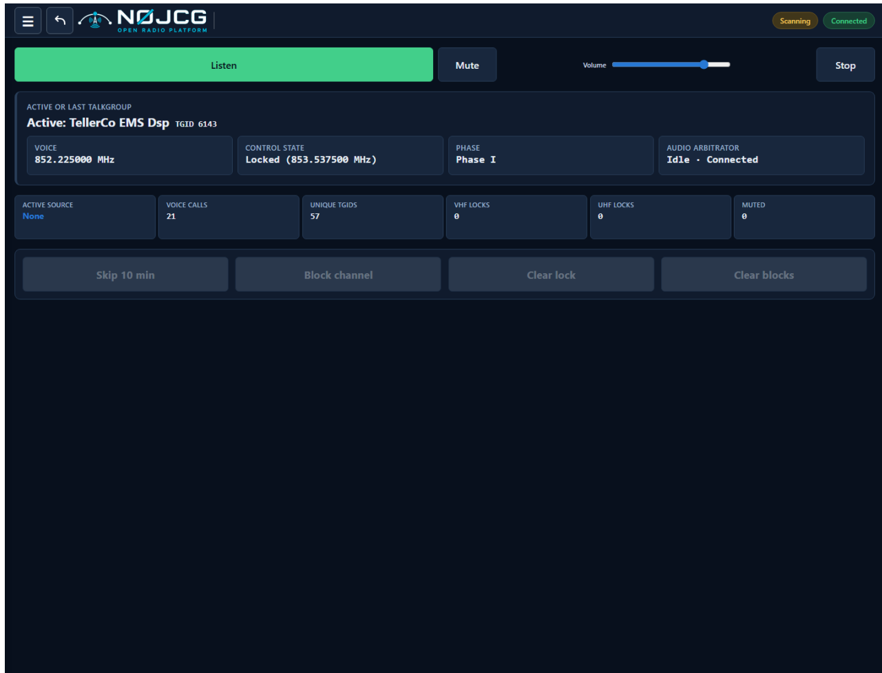
Current NOJCG Scanner dark-theme dashboard
