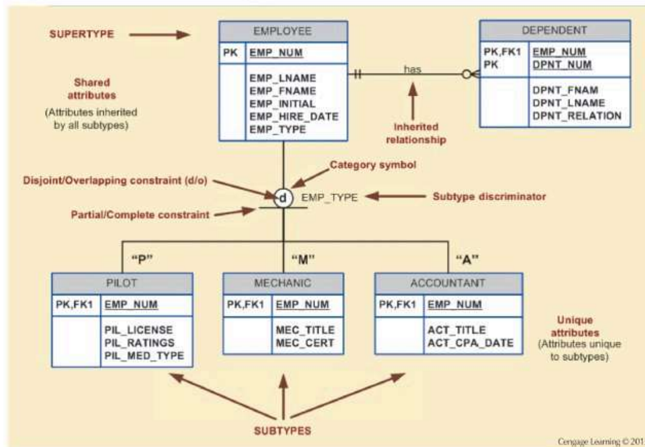
Figure 5.2 - Specialization Hierarchy
