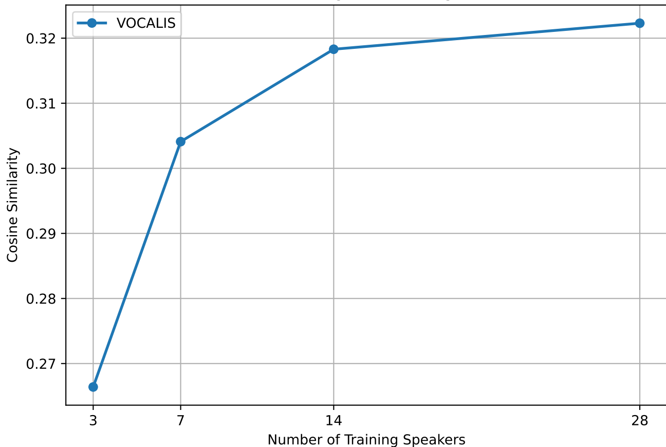
Training Data Scaling
