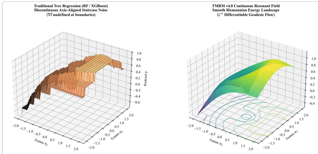
Figure 10.1: 3D Landscape Comparison: (Left) Decision Tree Regressors generate discontinuous staircase blocks where gradients are undefined; (Right) TMRM v4.0 constructs an infinitely smooth, differentiable Riemannian harmonic potential field.
