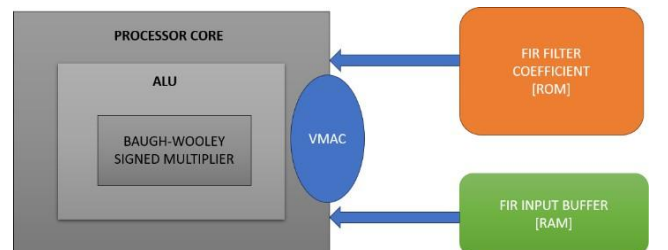
Fig. 2. FIR Filter Architecture
