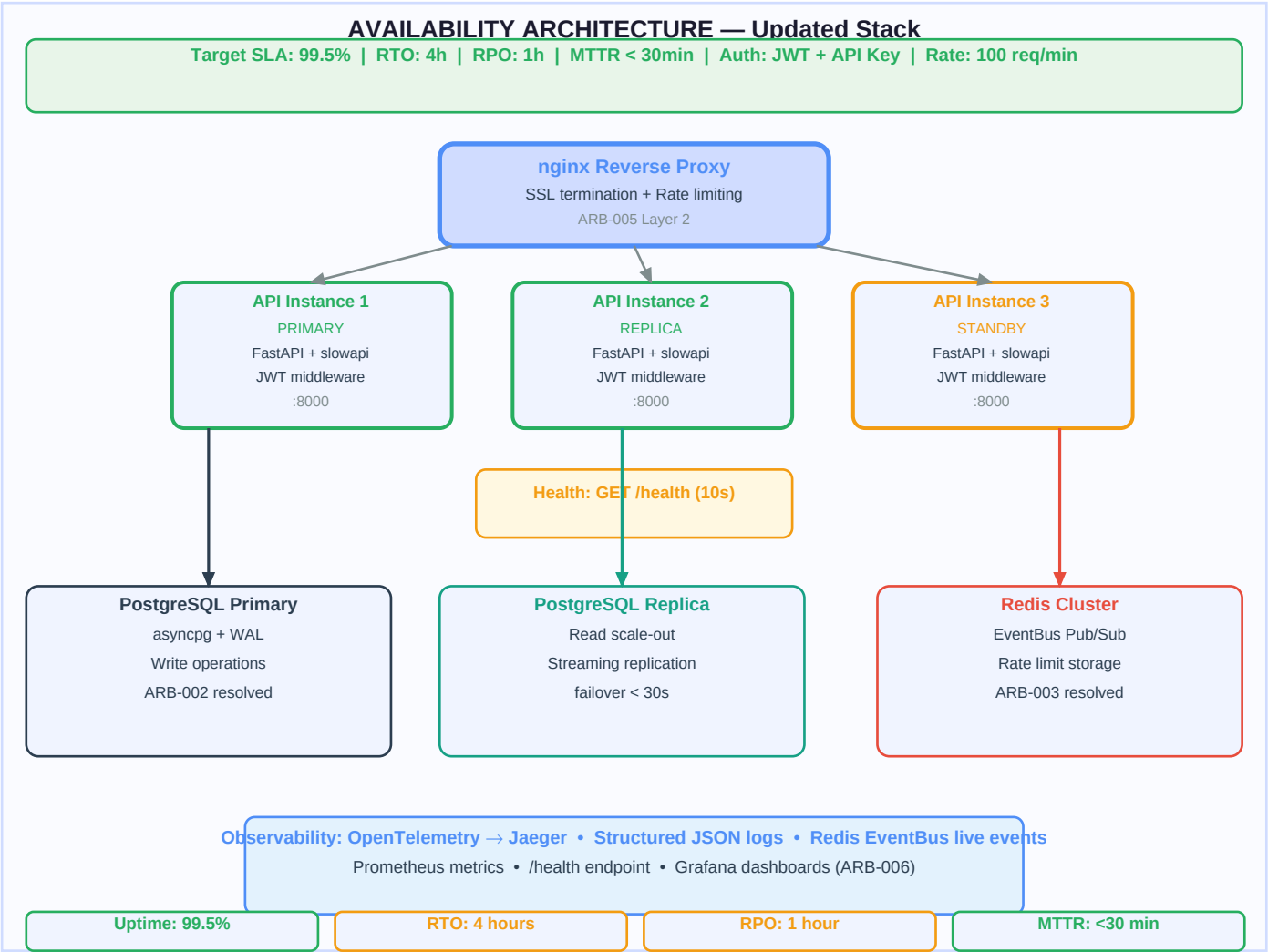
Figure 9: Availability Architecture
