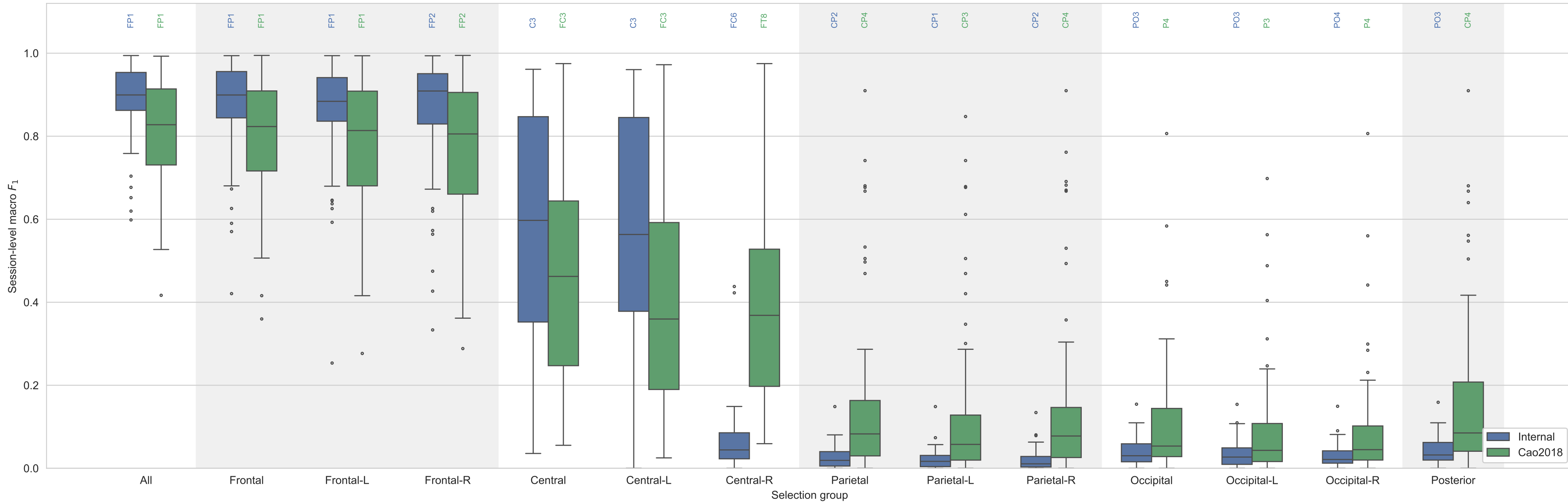
Best-channel-per-session macro F_1 by selection group (median center), Internal vs. Cao2018 (whole region shown alongside its own left/right hemisphere halves)
