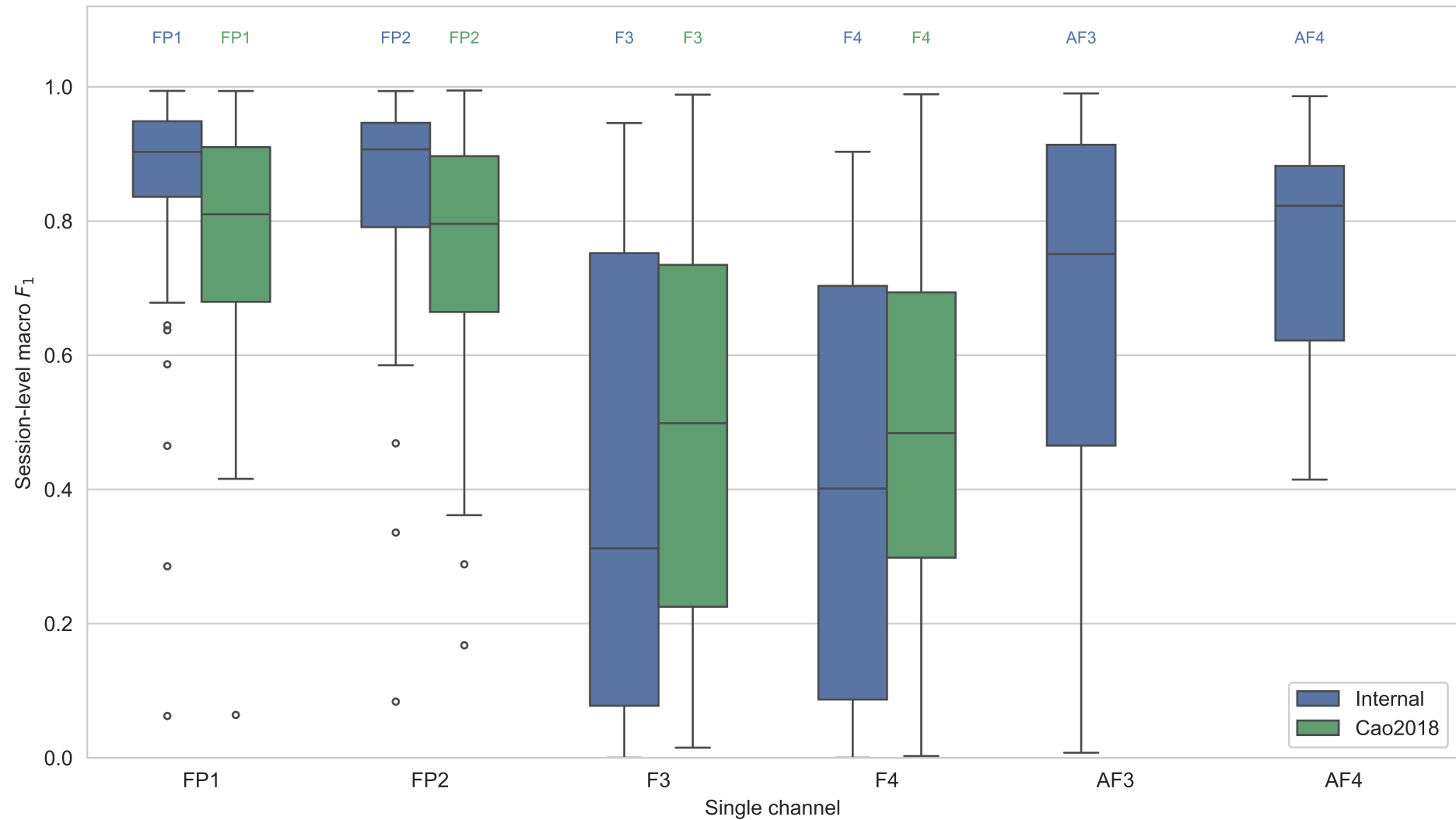
Single-channel-only session-level macro F_1 (median center), Internal vs. Cao2018
