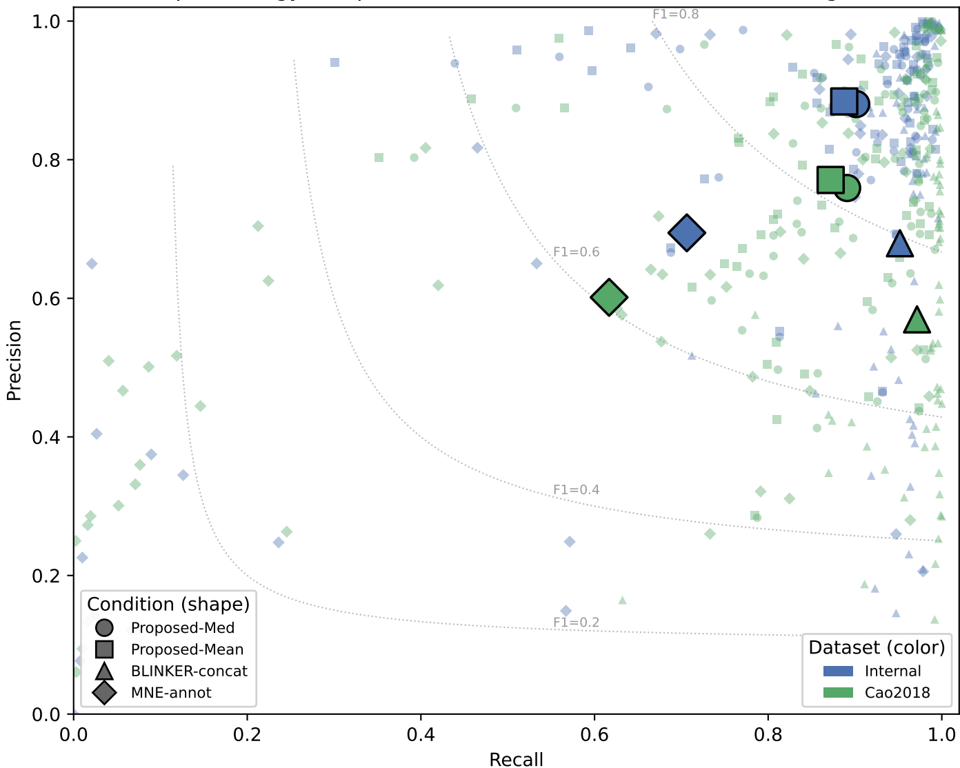
Per-session precision-recall operating points exp2 strategy comparison (Internal vs. Cao2018, all-channel gate)
