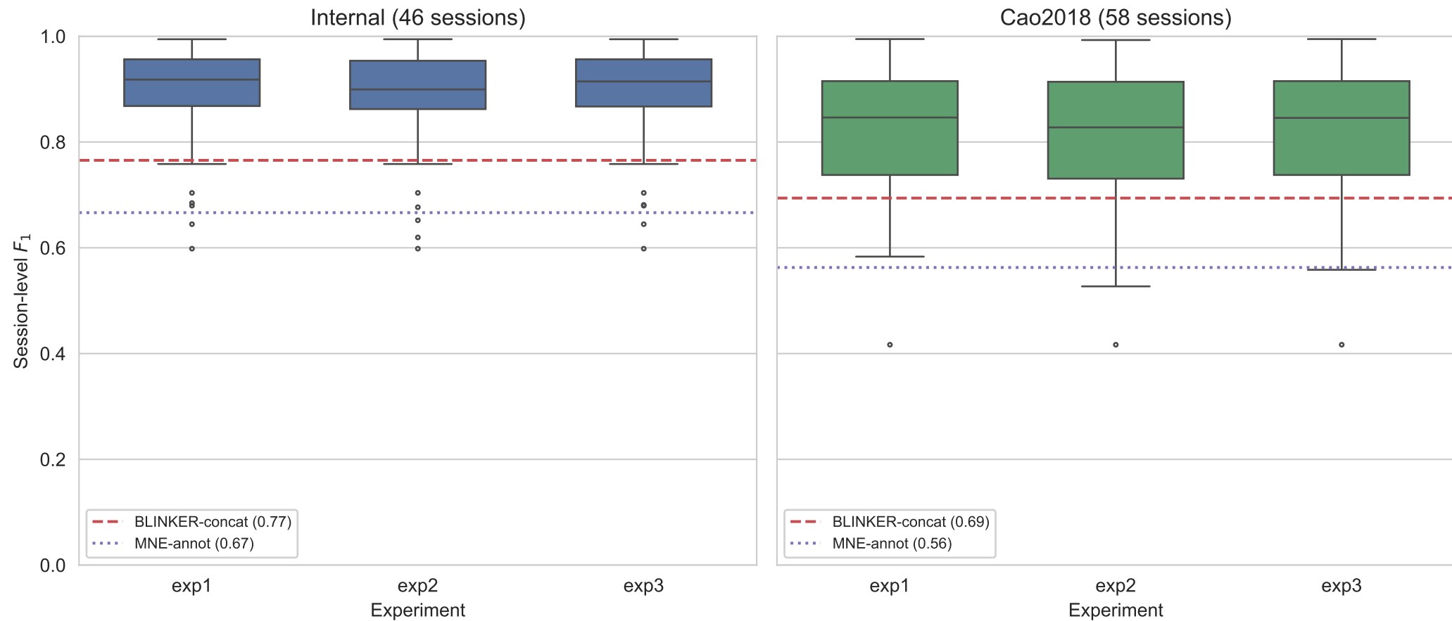
Proposed-Med session-level F_1 across experiments (best channel per session)
