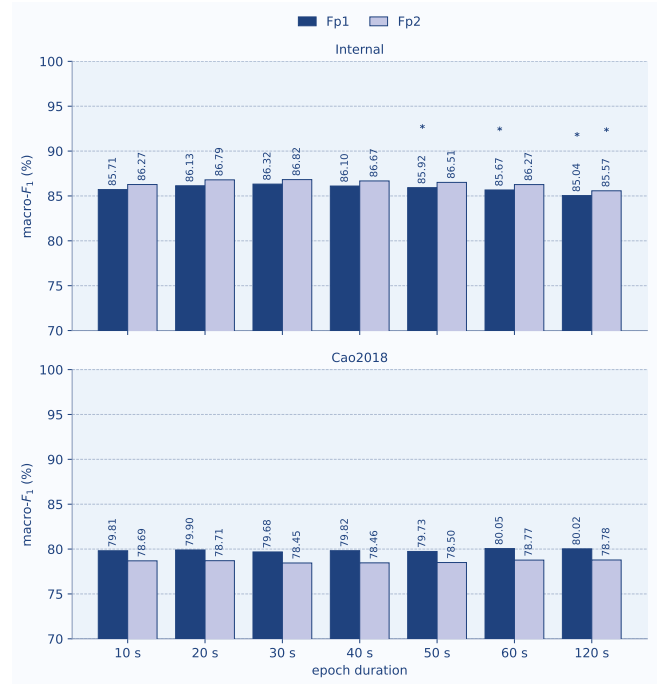
FIGURE 7. Macro-averaged F_1 of Proposed-approach across epoch durations, on the full 32-channel montage, for Fp1 and Fp2 (Experiment 1's two consistently best-performing electrodes) reported separately: Internal (top row) and Cao2018 (bottom row). Durations of 10, 20, 30 (reference), 40, 50, 60 and 120 seconds were tested, and an asterisk marks the durations that differ significantly from the 30 s reference after Bonferroni correction.
