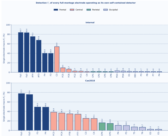
FIGURE 5. Detection F_1 of every electrode in the four curated anatomical regions operating as its own self-contained detector, in which the complete Stage A–Stage C pipeline was rerun on that one electrode alone, coloured by scalp region.
