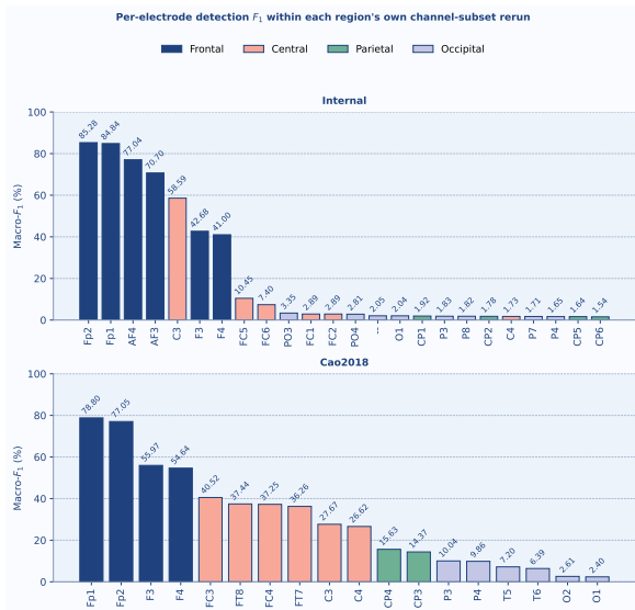
FIGURE 3. Per-electrode detection F_1 within each region's own channel-subset rerun, coloured by scalp region. Each bar is one electrode scored inside that region's own self-contained subset run.
