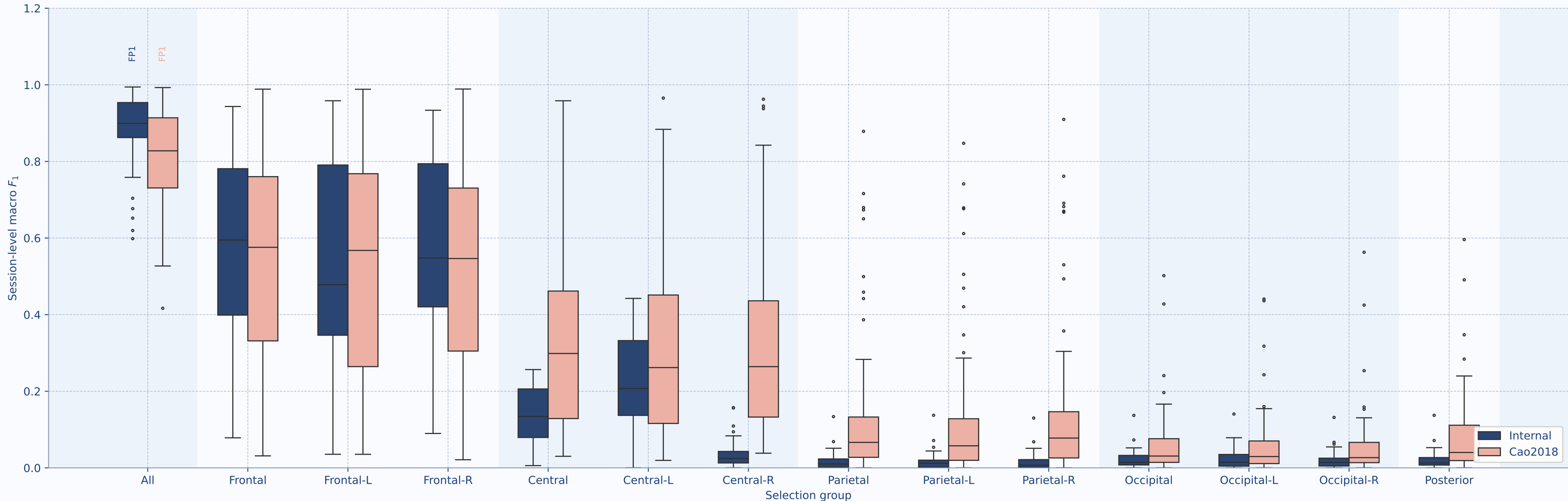
Session-level macro F_1 by selection group (median center), Internal vs. Cao2018 (All: best-channel-per-session; every other group: region-mean across its electrodes; whole region shown alongside its own left/right hemisphere halves)
