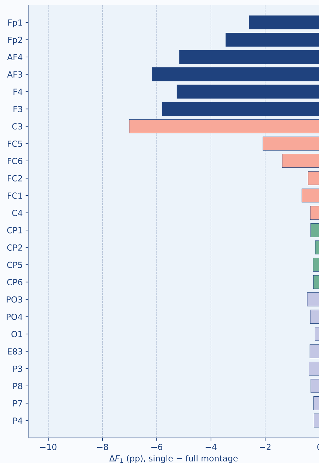
Internal
