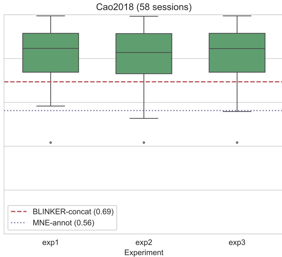
Proposed-Med session-level F_1 across experiments (best channel per session)
