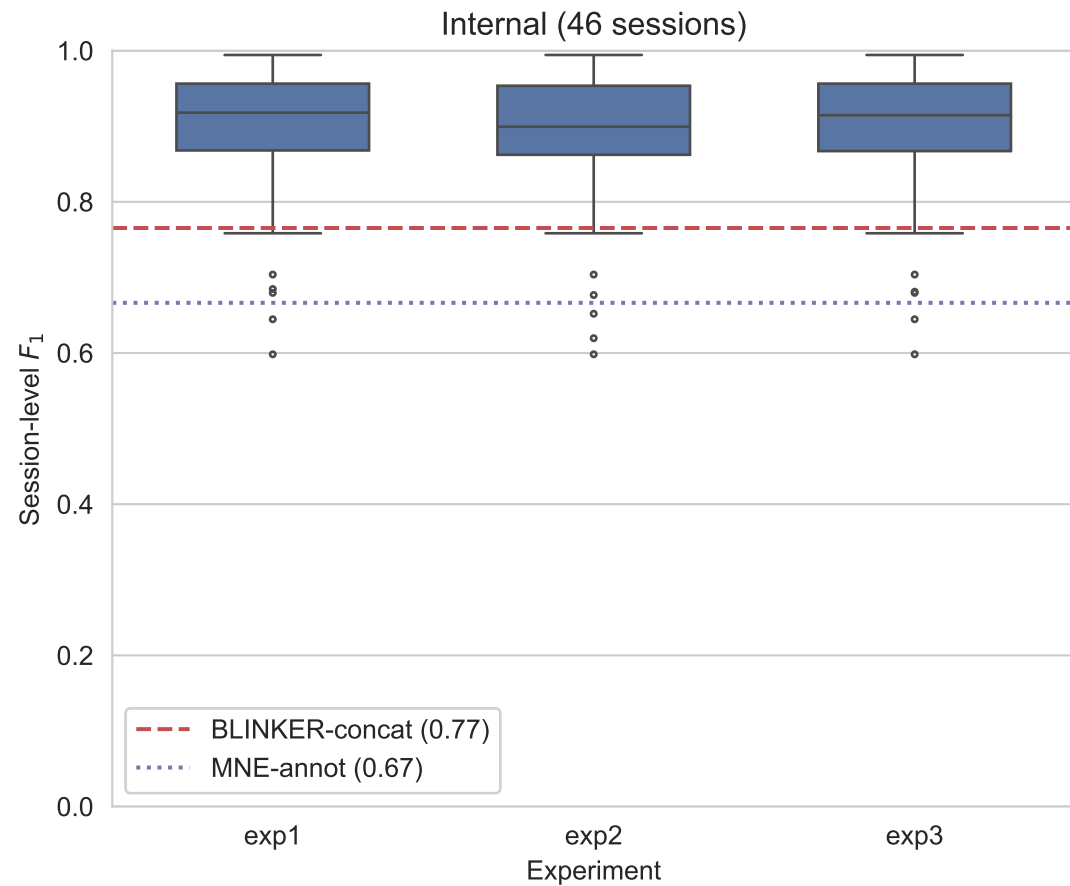
Proposed-Med session-level F_1 across experiments (best channel per session)
