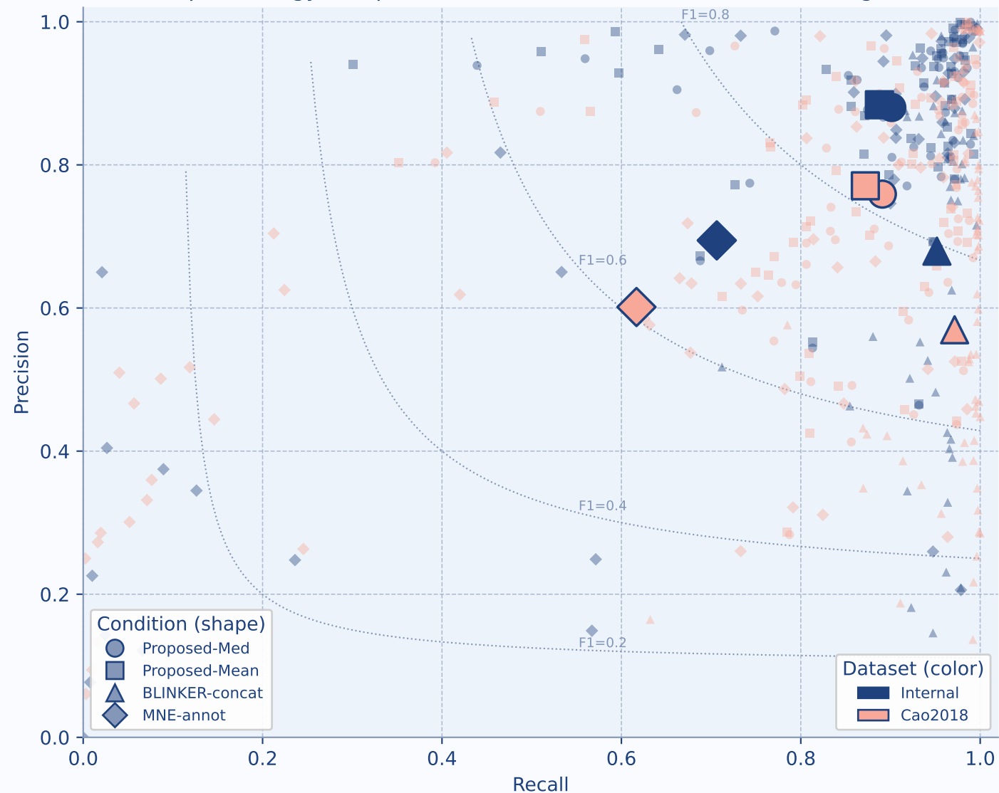
Per-session precision-recall operating points exp2 strategy comparison (Internal vs. Cao2018, all-channel gate)
