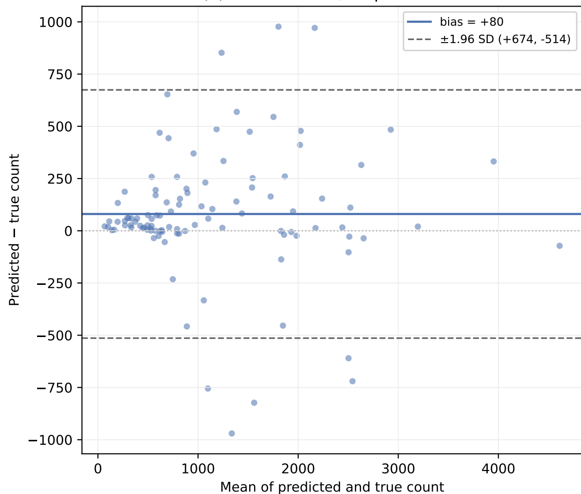
(b) Bland-Altman, Proposed-Med
