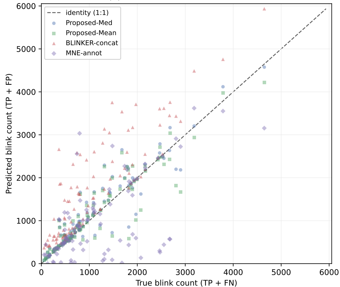
(a) Predicted vs. true event count
