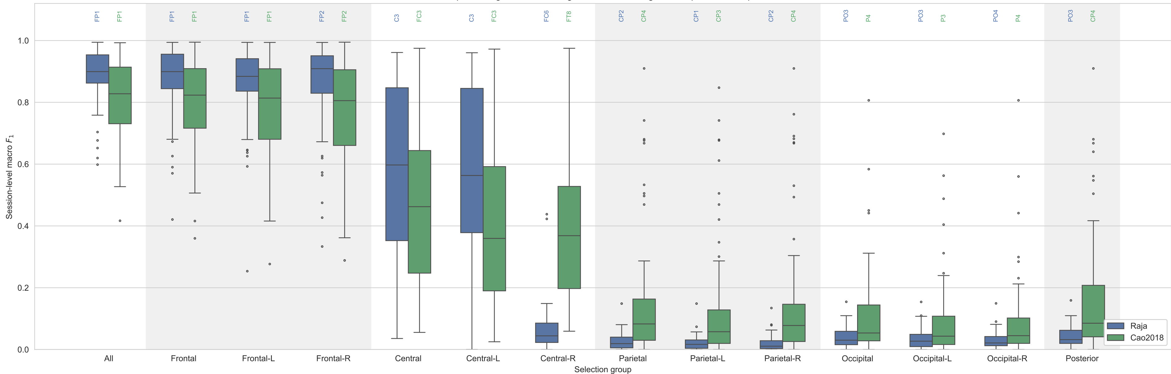
Best-channel-per-session macro F_1 by selection group (median center), Raja vs. Cao2018 (whole region shown alongside its own left/right hemisphere halves)
