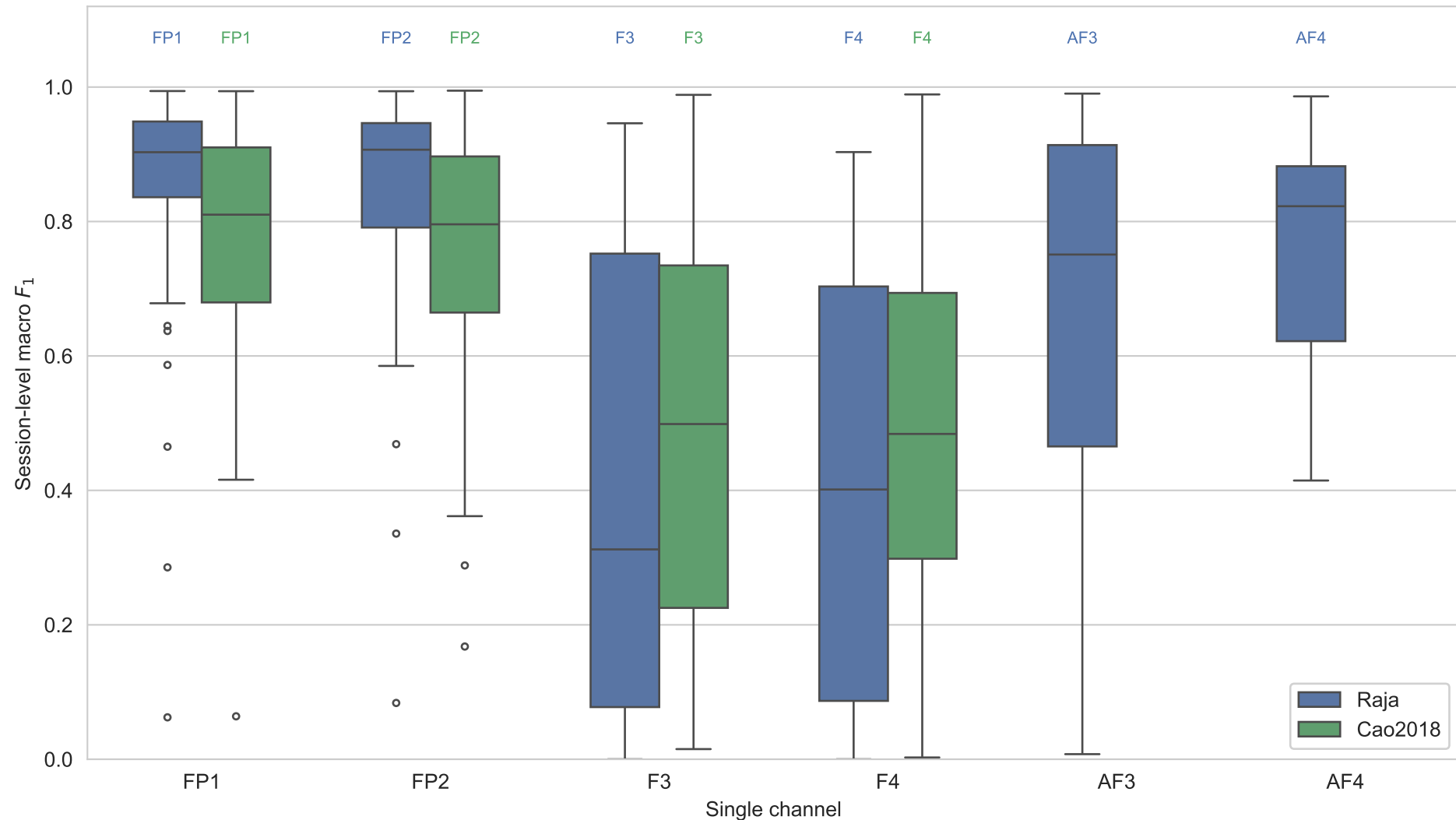
Single-channel-only session-level macro F_1 (median center), Raja vs. Cao2018
