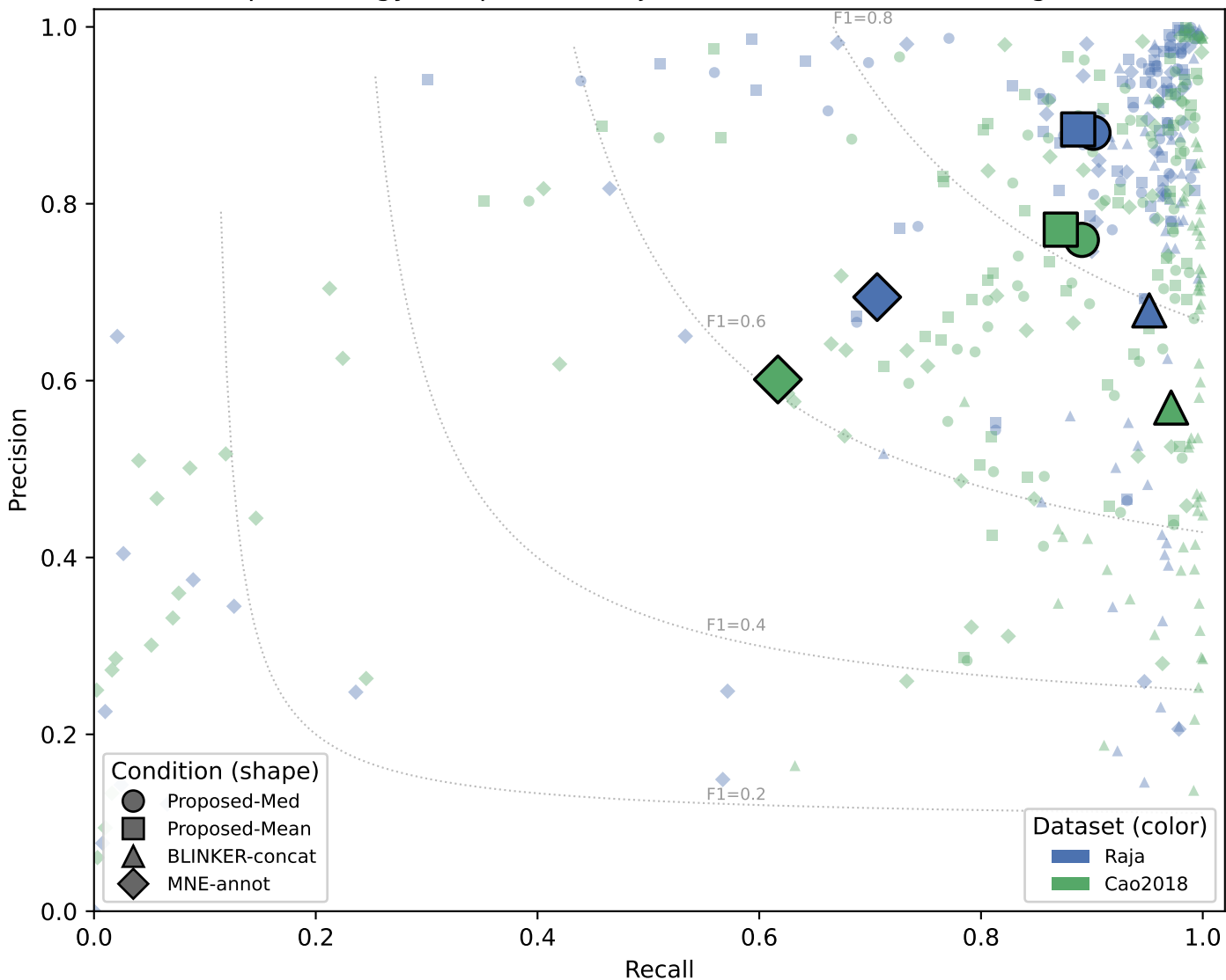
Per-session precision-recall operating points exp2 strategy comparison (Raja vs. Cao2018, all-channel gate)
