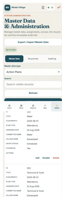
Admin mobile Master Data: desktop columns become stacked key/value fields.
