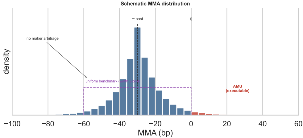
Figure 3: Schematic MMA distribution. The dashed rectangle over (-2\text{cost}', 0) is the no-information benchmark implied by the no-AMU band (uniform quoting), with \text{cost}' \equiv \text{cost} - \frac{1}{2}(F_{ask} - F_{bid})e^{-rT} . Competitive quoting instead concentrates the mode at -\text{cost}' , the symmetric equilibrium of the conjugate forward/backward paths; the mass that crosses zero into positive territory is the AMU. Schematic, illustrative levels.
