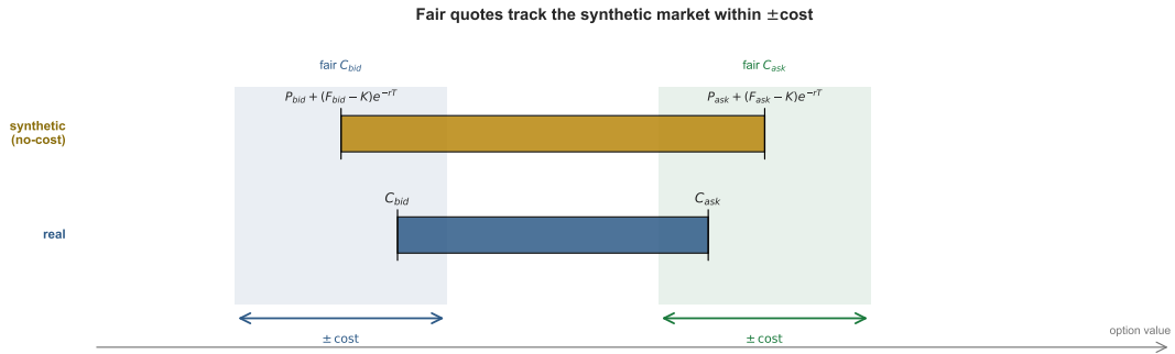
Figure 2: No AMU requires each real quote to track its matching synthetic quote within \pm \text{cost}' (the half-width \text{cost}' \equiv \text{cost} - \frac{1}{2}(F_{ask} - F_{bid})e^{-rT} ). The band centres are the frictionless (no-cost) synthetic prices P_{bid} + (F_{bid} - K)e^{-rT} and P_{ask} + (F_{ask} - K)e^{-rT} ; the cushion around each is \pm \text{cost}' . As frictions shrink, the real market is squeezed onto the synthetic market. Schematic, illustrative levels.
