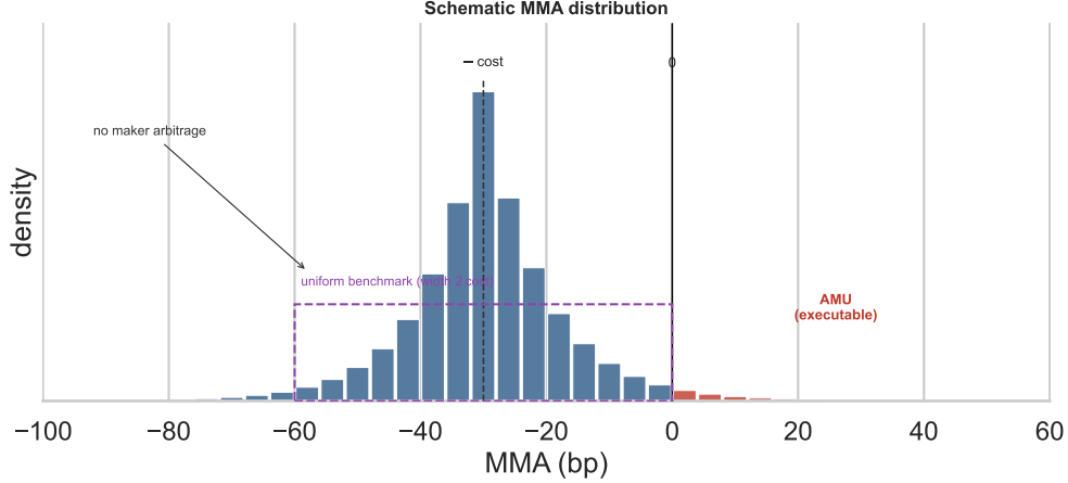
Figure 3: Schematic MMA distribution. The dashed rectangle over (-2\text{cost}, 0) is the no-information benchmark implied by the no-AMU band (uniform quoting). Competitive quoting instead concentrates the mode at -\text{cost} , the symmetric equilibrium of the conjugate forward/backward paths; the mass that crosses zero into positive territory is the executable AMU. Schematic, illustrative levels.
