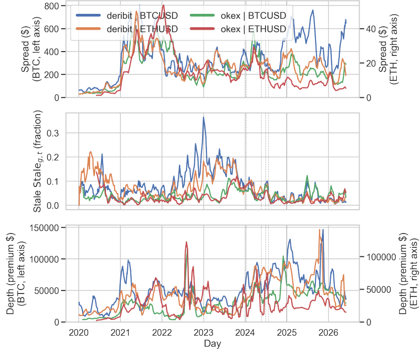
Figure 1: Raw quote statistics over time by exchange and underlying, smoothed with a trailing 1-month rolling mean and aggregated over strike and maturity. Bid–ask spread in dollars ( \text{Spr}_{g,t}^{\$} ); the stale-quote fraction \text{Stale}_{g,t} ; and the quote depth in premium dollars (the resting size times the contract size times the option price, i.e. the dollar value of the resting quote). Dashed vertical lines mark the 2024 events: BTC ETP approval (10 Jan), ETH ETF approval (23 May), MiCA stablecoin rules (30 Jun), ETH ETF trading (23 Jul), and MiCA CASP rules (30 Dec).
