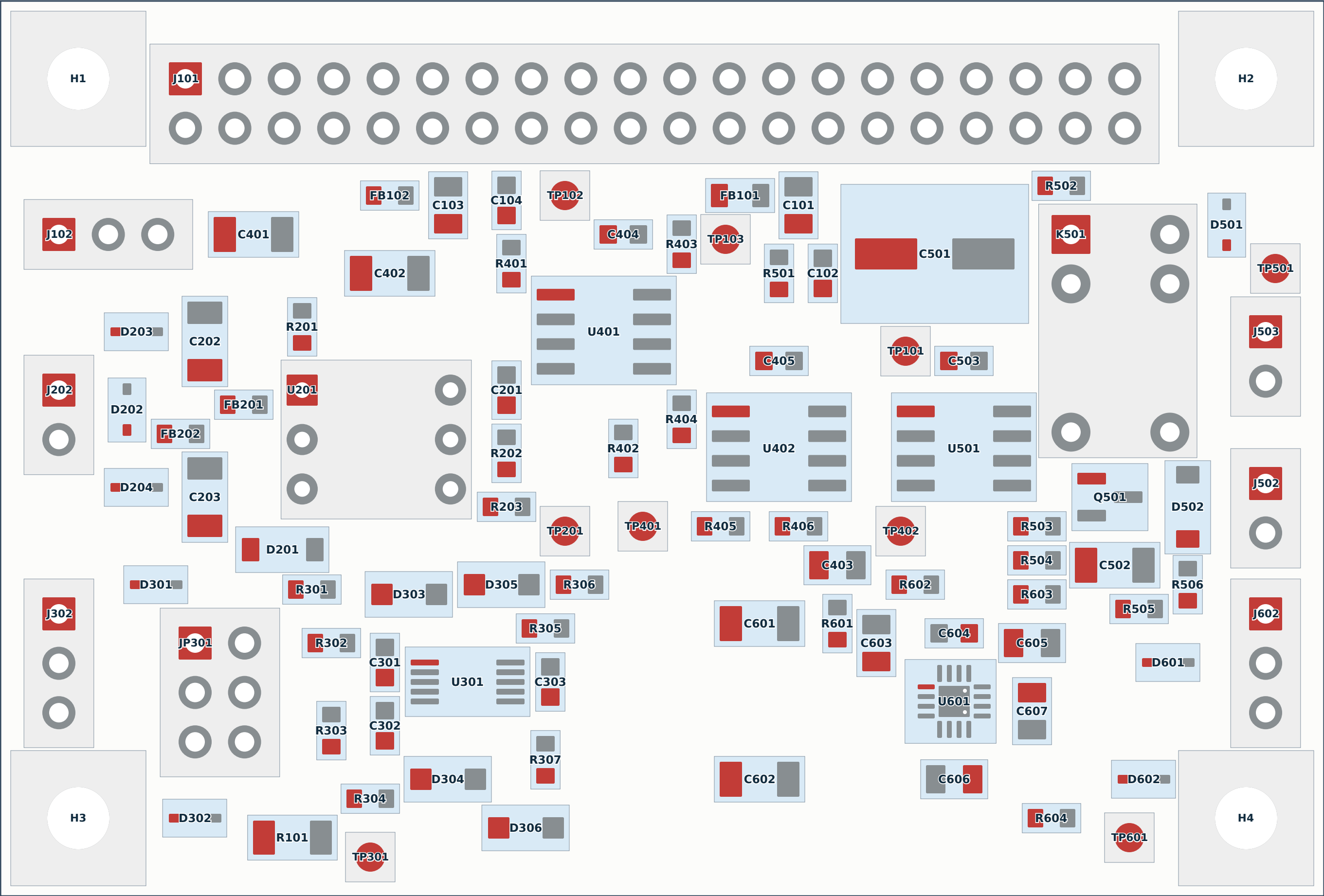
Top view, 68 x 46 mm. Pin numbers follow the KiCad footprint; this drawing is not JLCPCB's placement preview.
