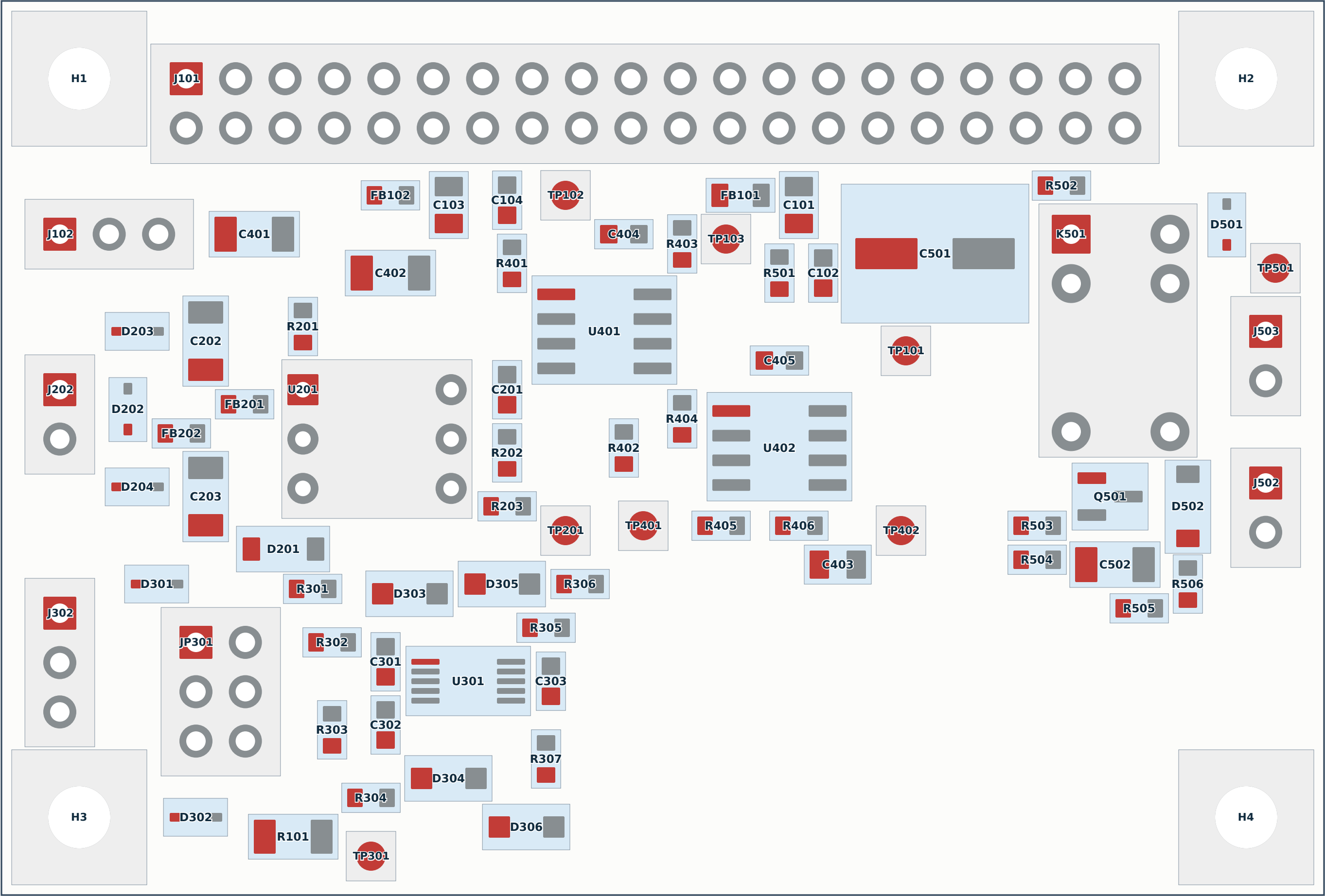
Top view, 68 × 46 mm. Pin numbers follow the KiCad footprint; this drawing is not JLCPCB’s placement preview.
