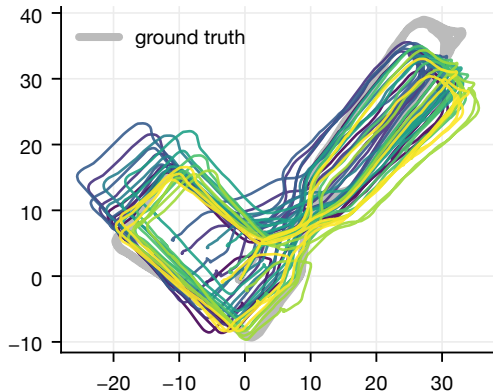
(b) ordinary network (yaw-augmented)
